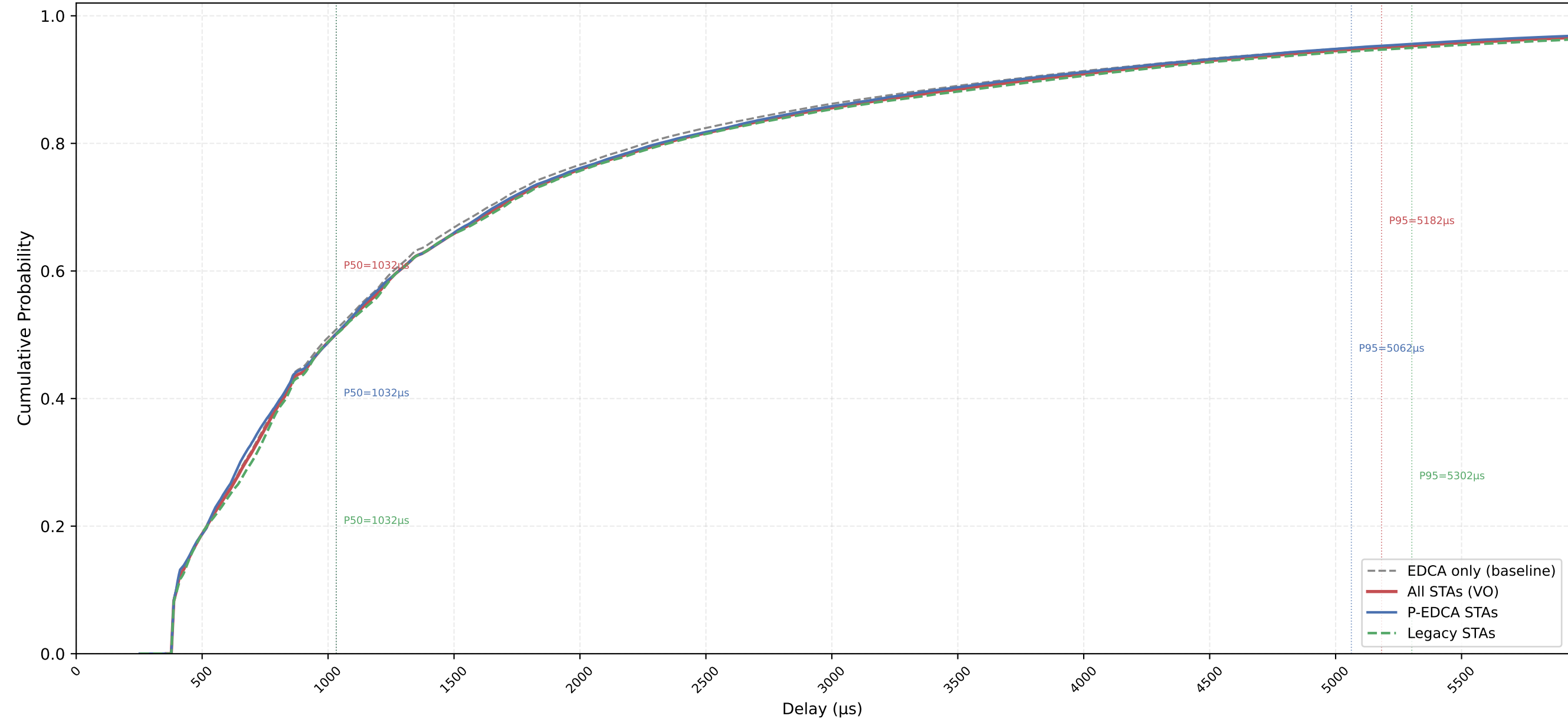
VO Delay CDF — P-EDCA / Legacy / All | CWds=0 × QSRC=4 × PSRC=2 nSta=30, nPedca=15/30, 0.5Mbps, avg of 10 runs
