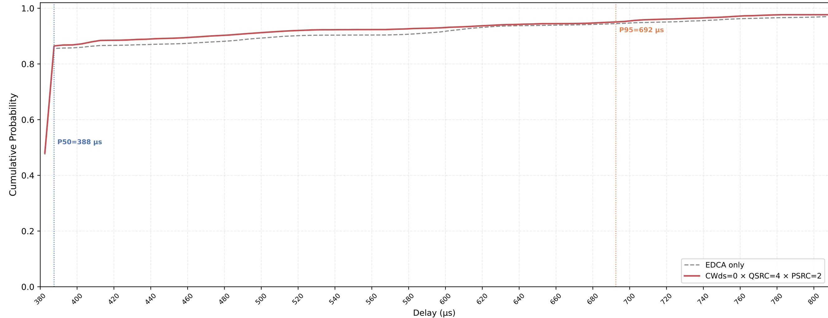
P-EDCA STA VO Delay CDF — CWds=0 × QSRC=4 × PSRC=2 nSta=30, nPedca=15, 0.1Mbps, avg of 10 runs
