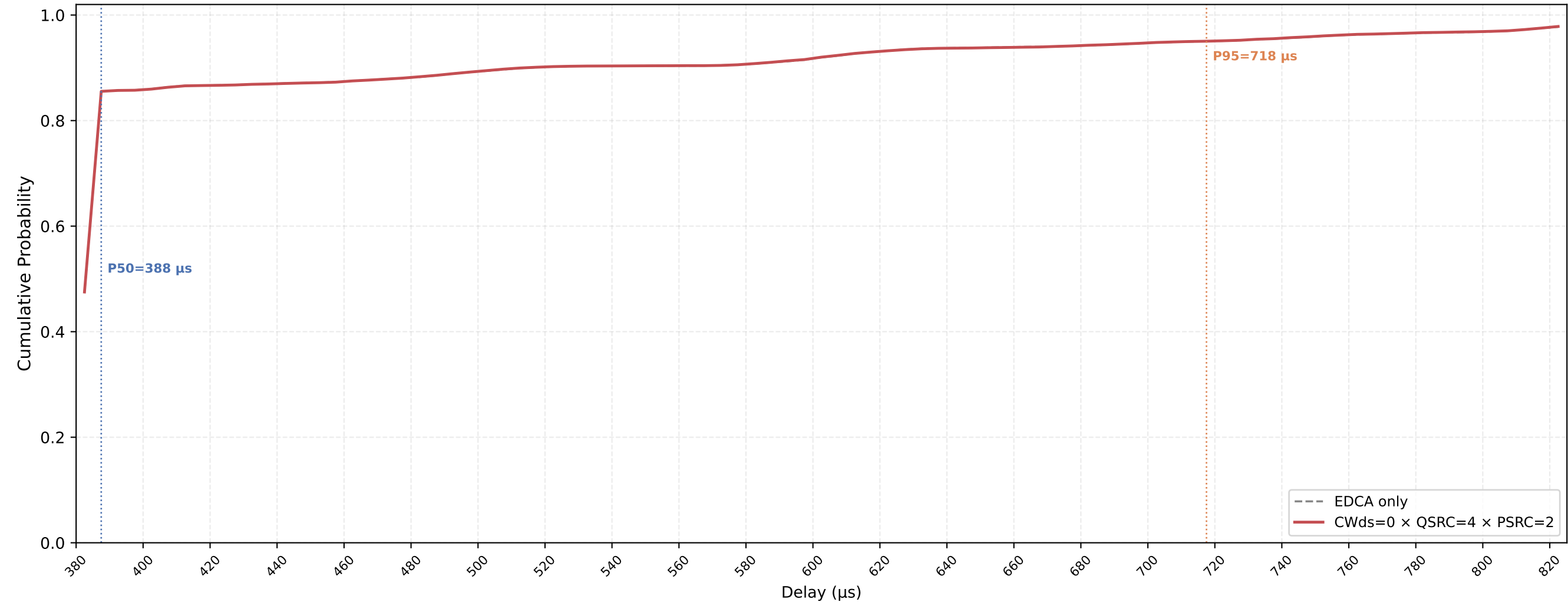
VO (all STAs) Delay CDF — CWds=0 × QSRC=4 × PSRC=2 nSta=30, nPedca=5, 0.1Mbps, avg of 10 runs
