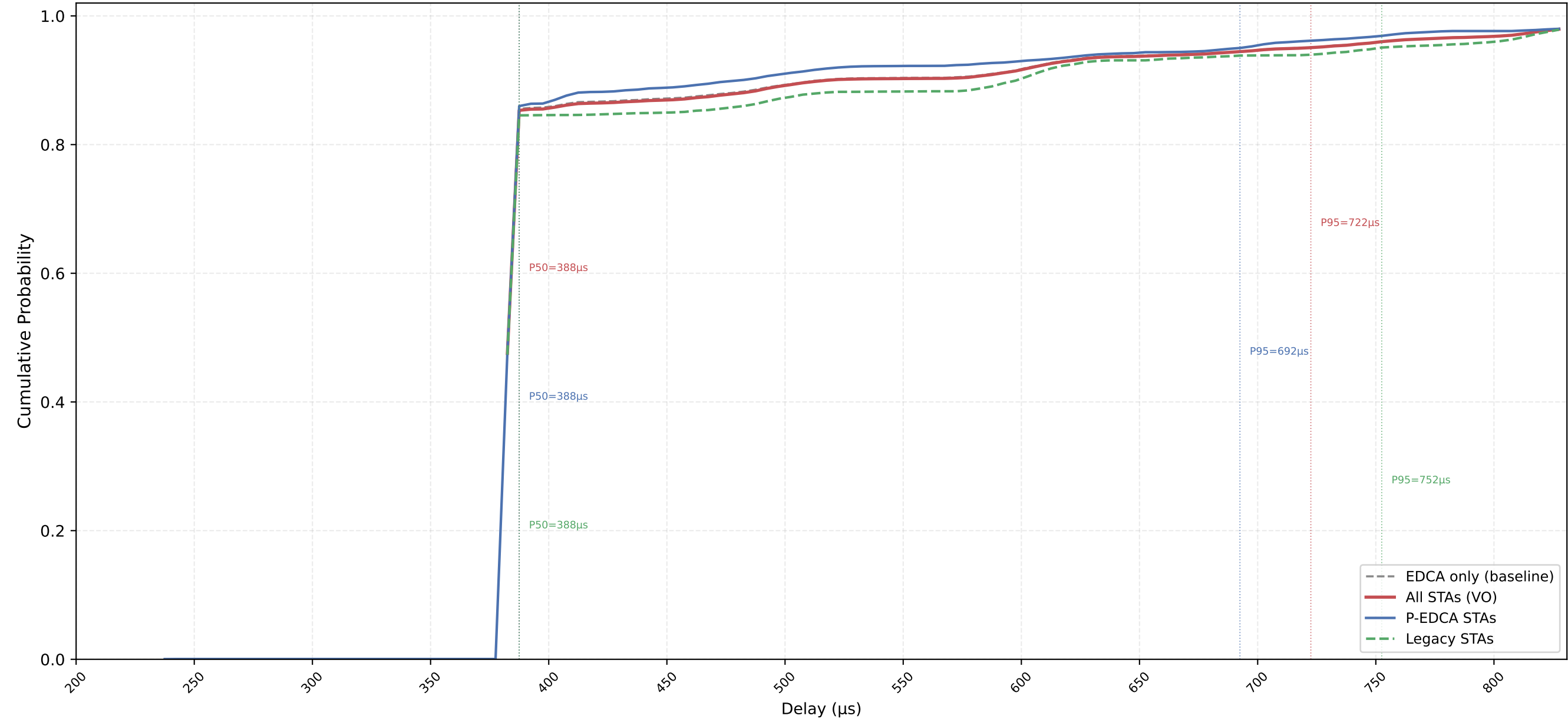
VO Delay CDF — P-EDCA / Legacy / All | CWds=0 × QSRC=4 × PSRC=3 nSta=30, nPedca=15/30, 0.1Mbps, avg of 10 runs
