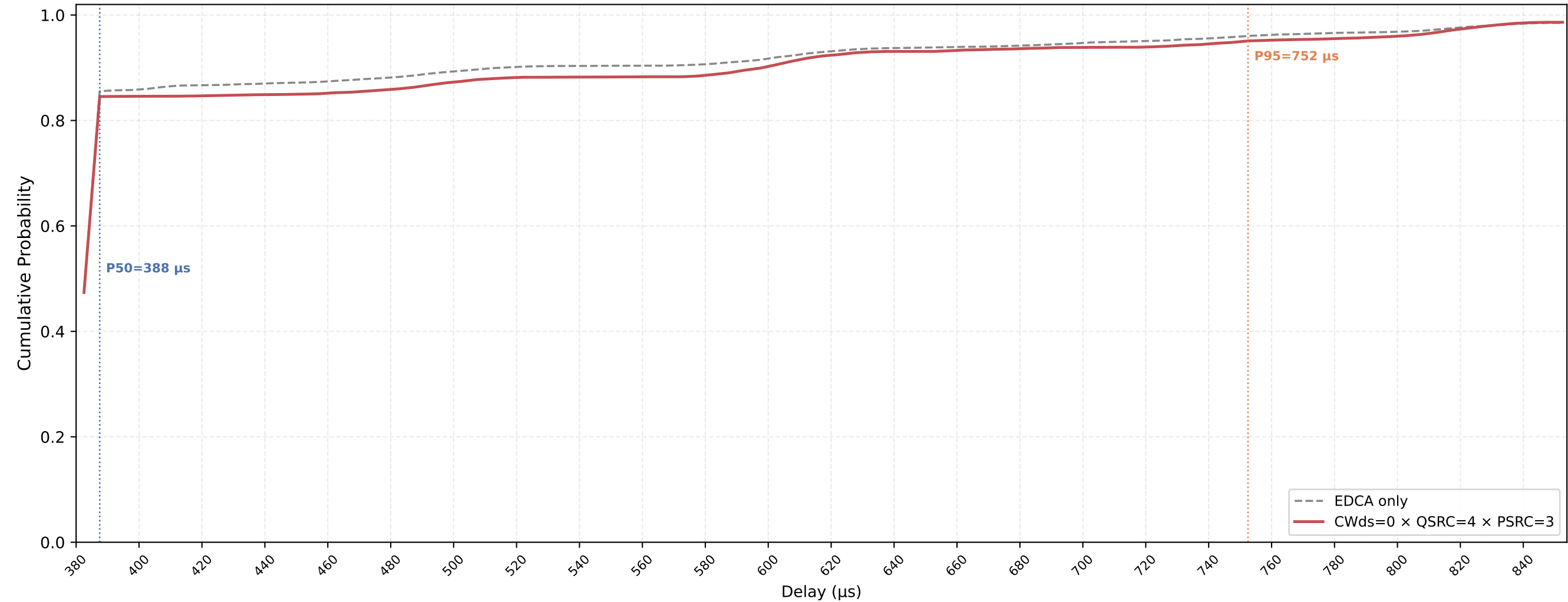
Legacy STA VO Delay CDF — CWds=0 × QSRC=4 × PSRC=3 nSta=30, nPedca=15, 0.1Mbps, avg of 10 runs
