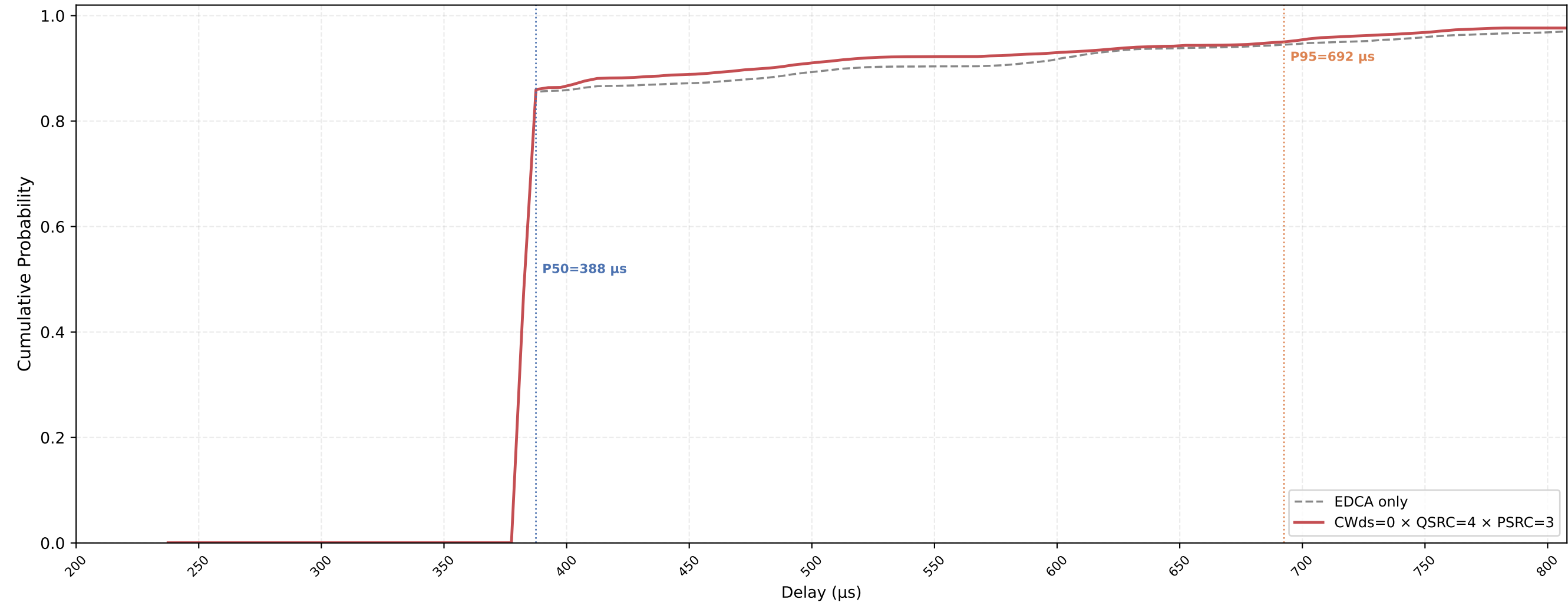
P-EDCA STA VO Delay CDF — CWds=0 × QSRC=4 × PSRC=3 nSta=30, nPedca=15, 0.1Mbps, avg of 10 runs
