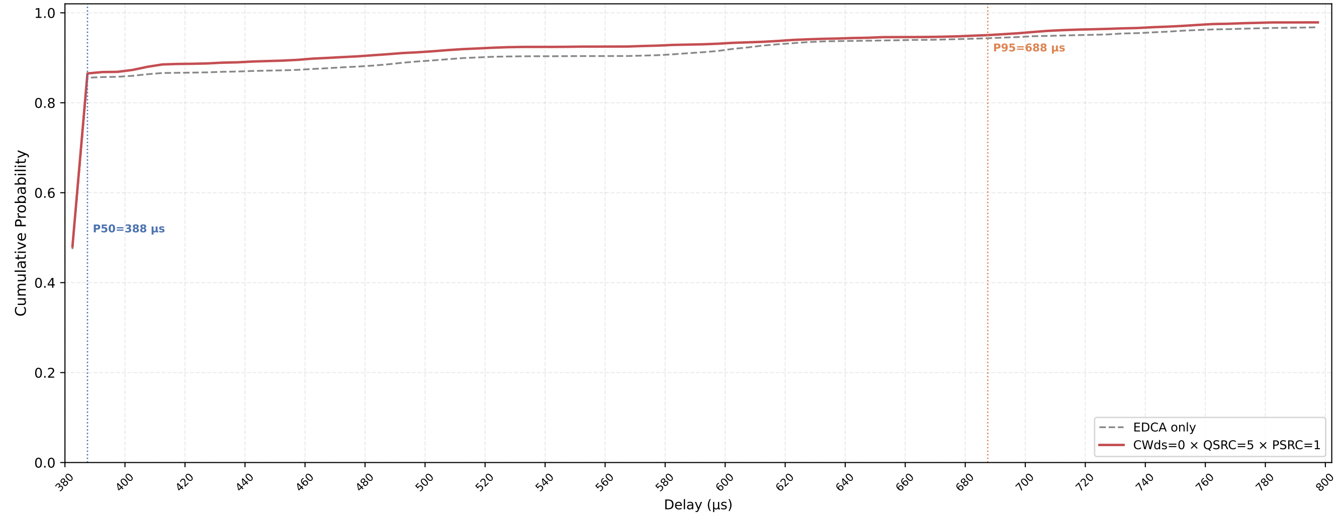
P-EDCA STA VO Delay CDF — CWds=0 × QSRC=5 × PSRC=1 nSta=30, nPedca=15, 0.1Mbps, avg of 10 runs
