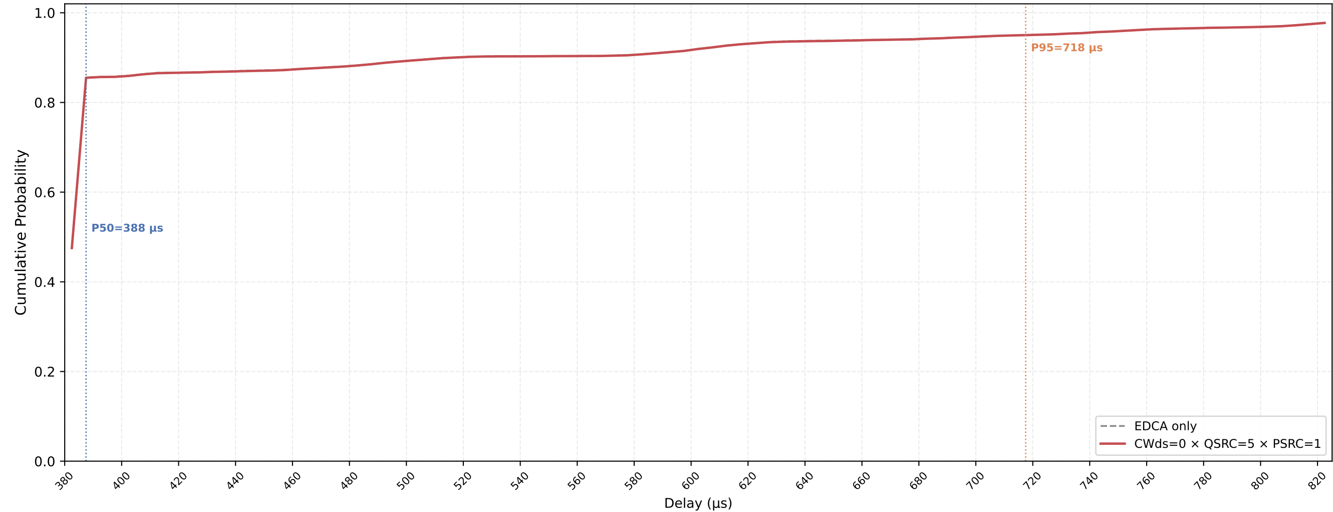
VO (all STAs) Delay CDF — CWds=0 × QSRC=5 × PSRC=1 nSta=30, nPedca=15, 0.1Mbps, avg of 10 runs
