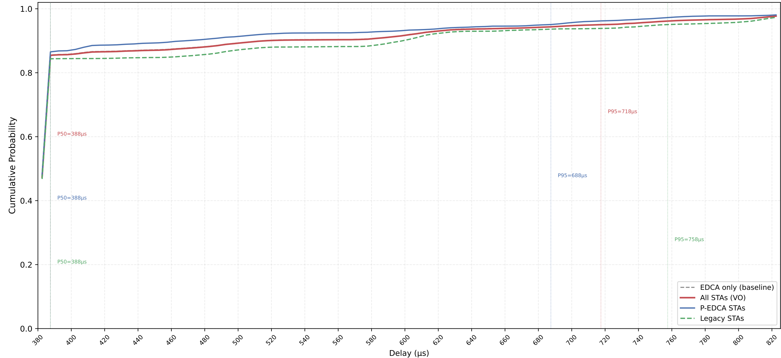
VO Delay CDF — P-EDCA / Legacy / All | CWds=0 × QSRC=5 × PSRC=2 nSta=30, nPedca=15/30, 0.1Mbps, avg of 10 runs
