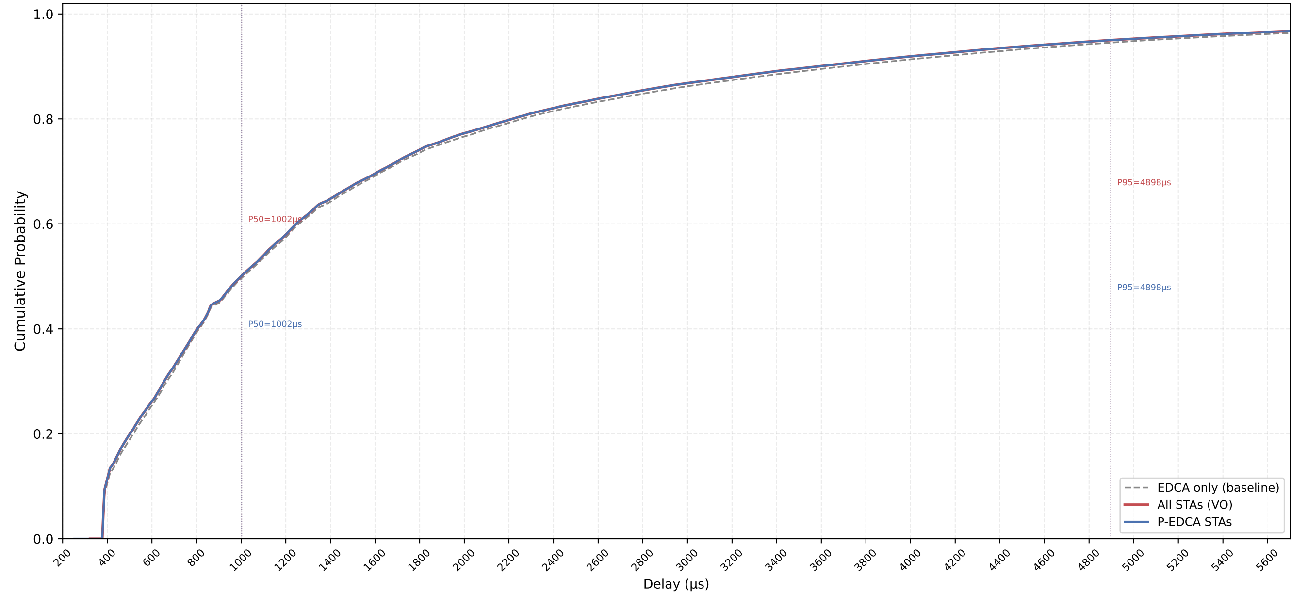
VO Delay CDF — P-EDCA / Legacy / All | CWds=0 × QSRC=5 × PSRC=2 nSta=30, nPedca=30/30, 0.5Mbps, avg of 10 runs
