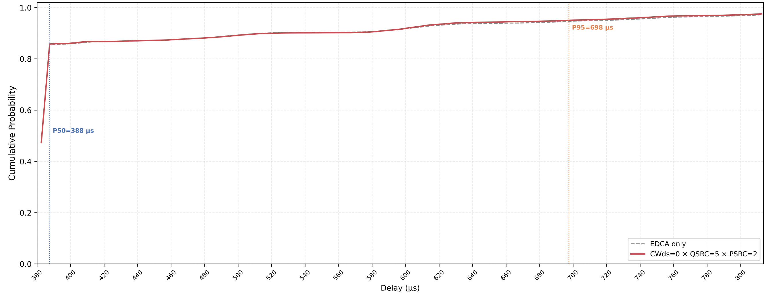
Legacy STA VO Delay CDF — CWds=0 × QSRC=5 × PSRC=2 nSta=30, nPedca=5, 0.1Mbps, avg of 10 runs
