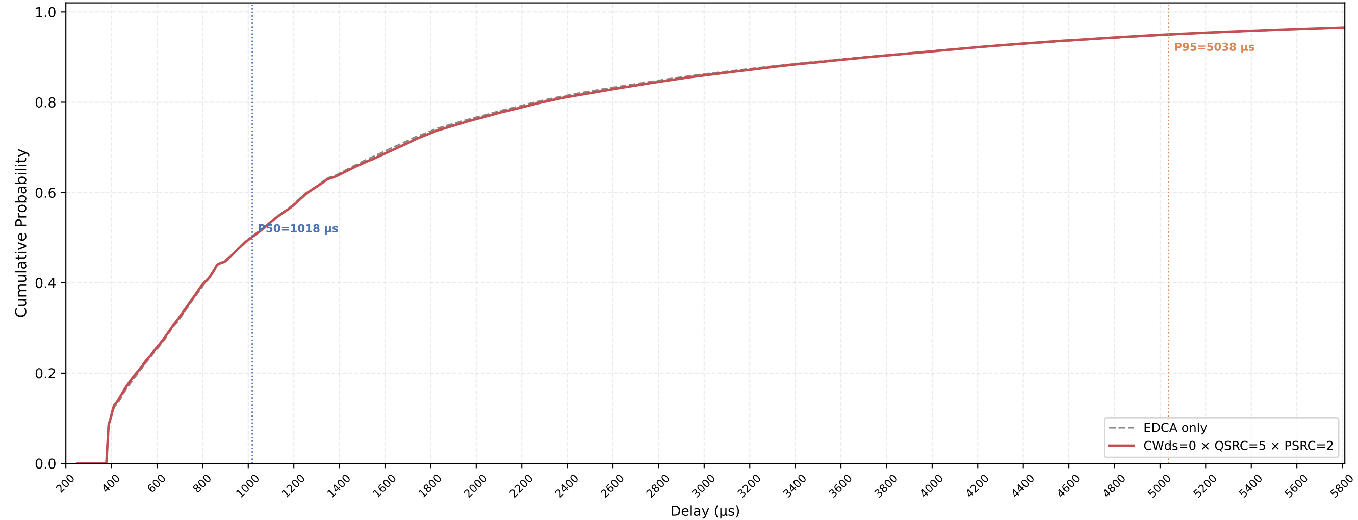
Legacy STA VO Delay CDF — CWds=0 × QSRC=5 × PSRC=2 nSta=30, nPedca=5, 0.5Mbps, avg of 10 runs
