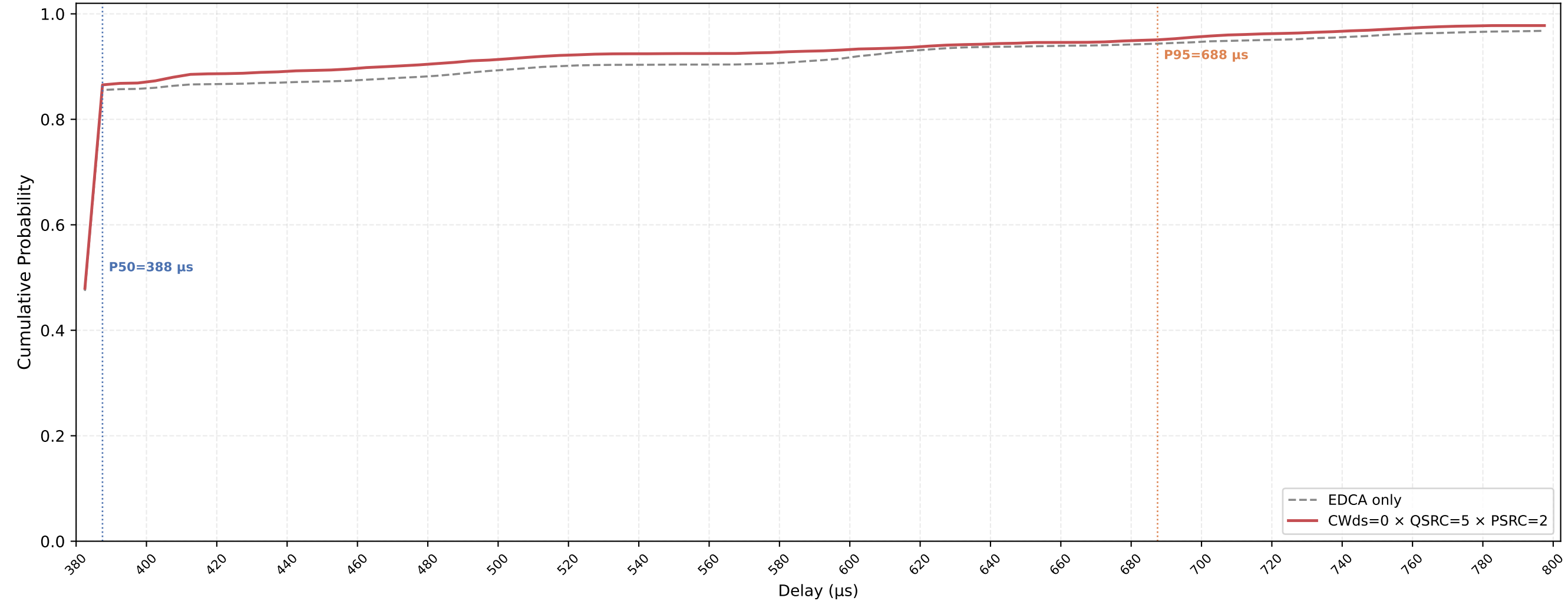
P-EDCA STA VO Delay CDF — CWds=0 × QSRC=5 × PSRC=2 nSta=30, nPedca=15, 0.1Mbps, avg of 10 runs
