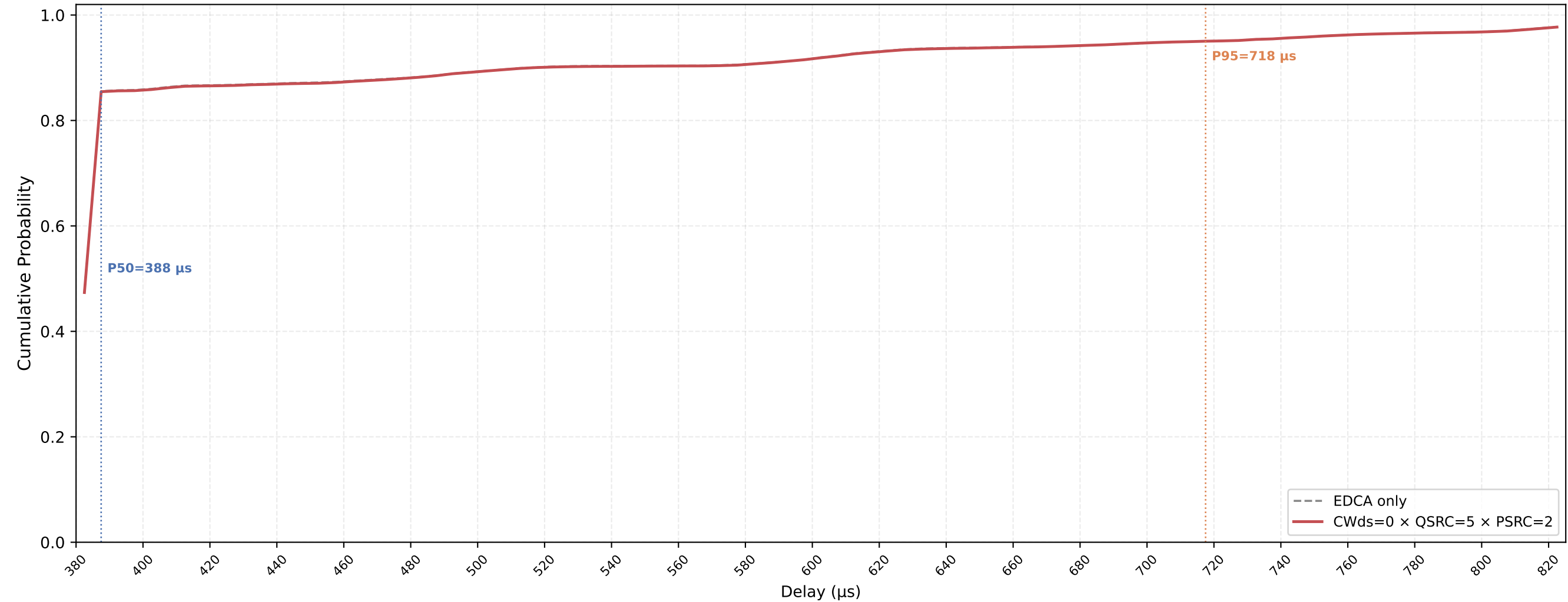
VO (all STAs) Delay CDF — CWds=0 × QSRC=5 × PSRC=2 nSta=30, nPedca=15, 0.1Mbps, avg of 10 runs
