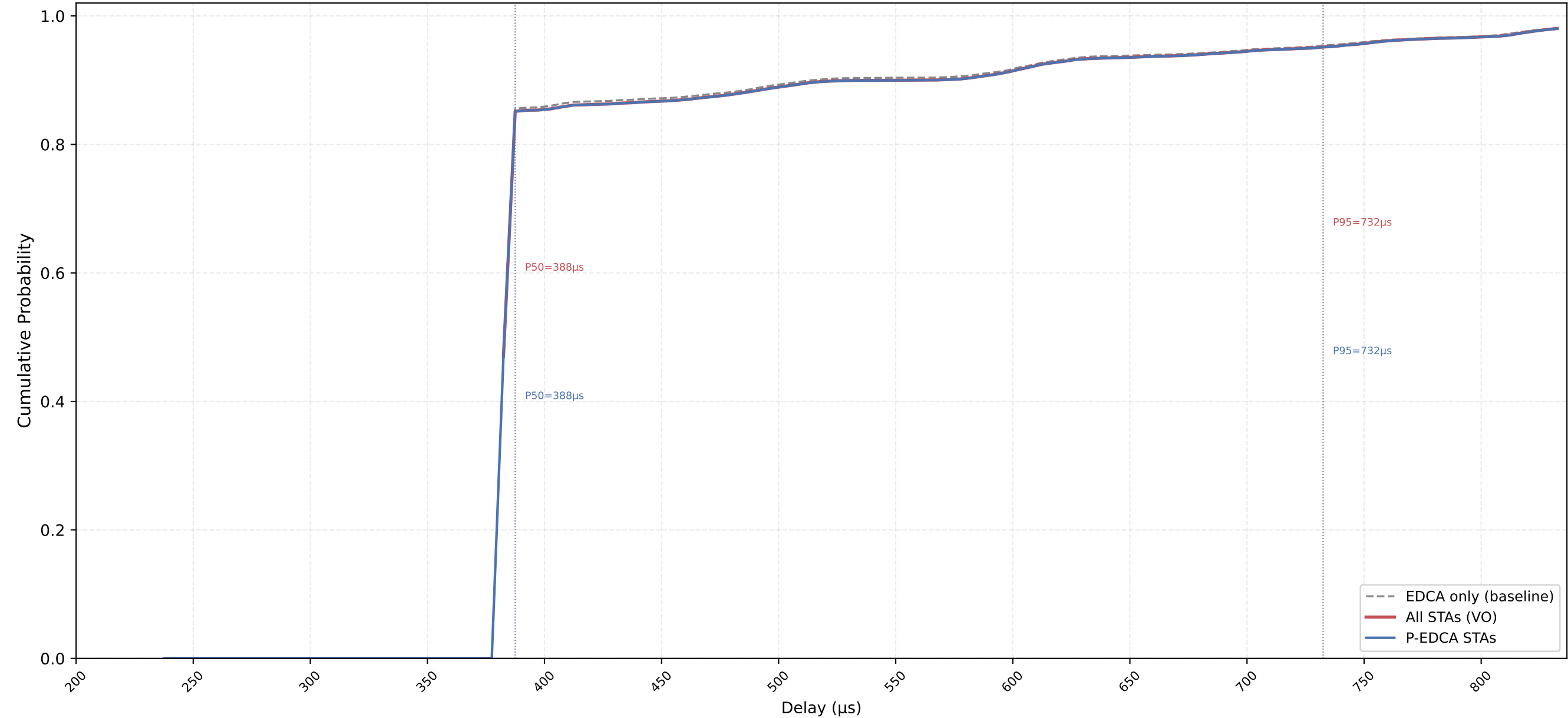
VO Delay CDF — P-EDCA / Legacy / All | CWds=0 × QSRC=5 × PSRC=3 nSta=30, nPedca=30/30, 0.1Mbps, avg of 10 runs
