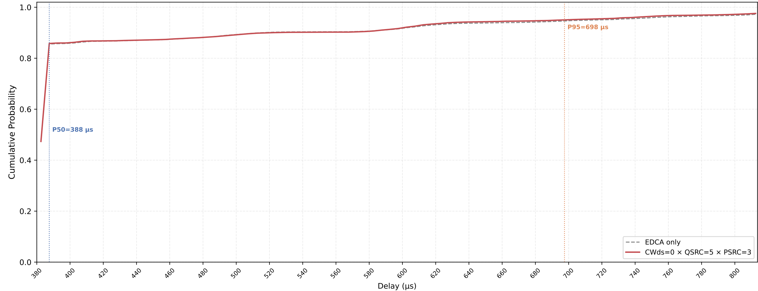
Legacy STA VO Delay CDF — CWds=0 × QSRC=5 × PSRC=3 nSta=30, nPedca=5, 0.1Mbps, avg of 10 runs
