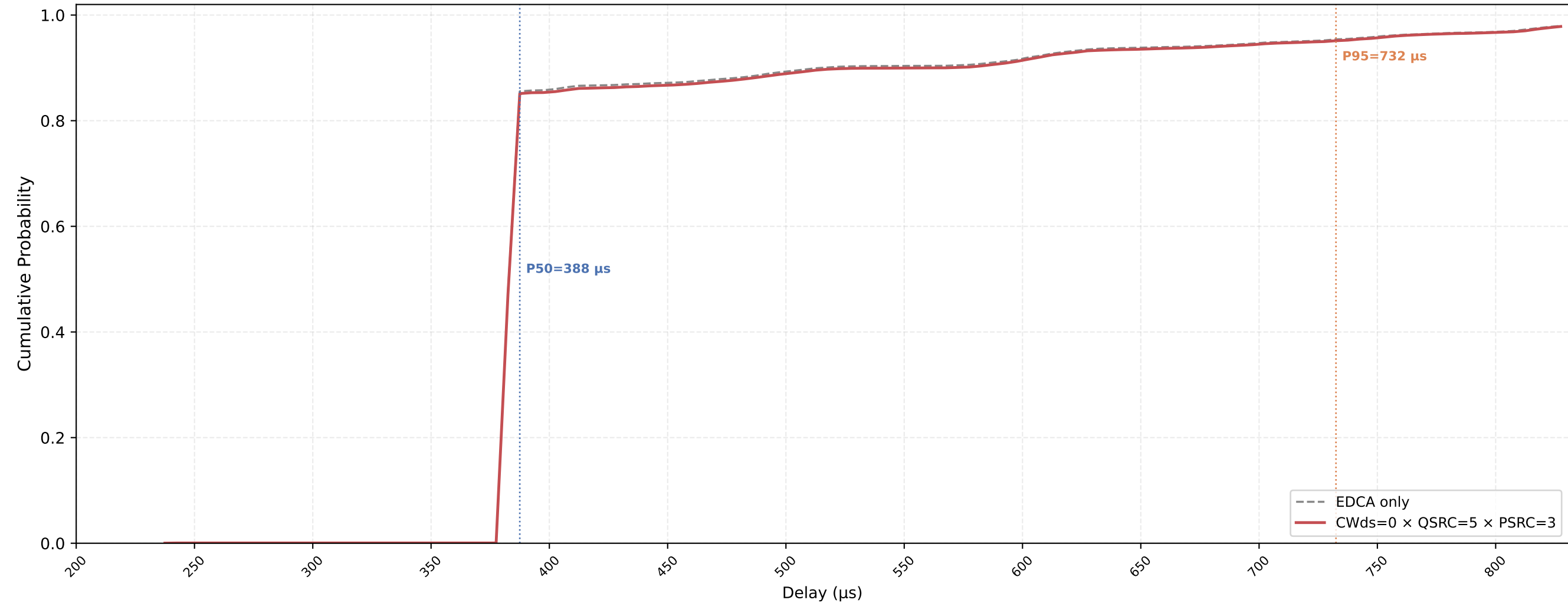
P-EDCA STA VO Delay CDF — CWds=0 × QSRC=5 × PSRC=3 nSta=30, nPedca=30, 0.1Mbps, avg of 10 runs
