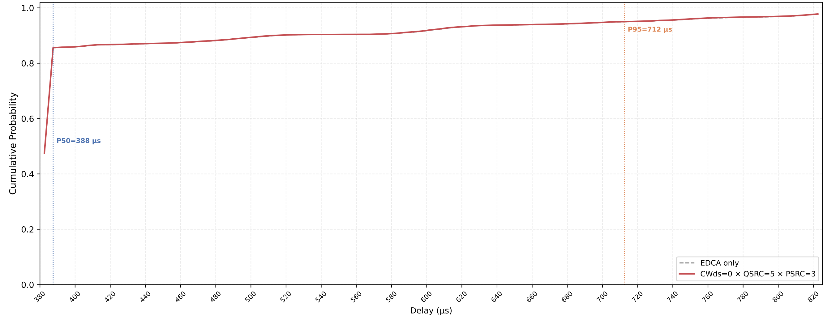
VO (all STAs) Delay CDF — CWds=0 × QSRC=5 × PSRC=3 nSta=30, nPedca=5, 0.1Mbps, avg of 10 runs
