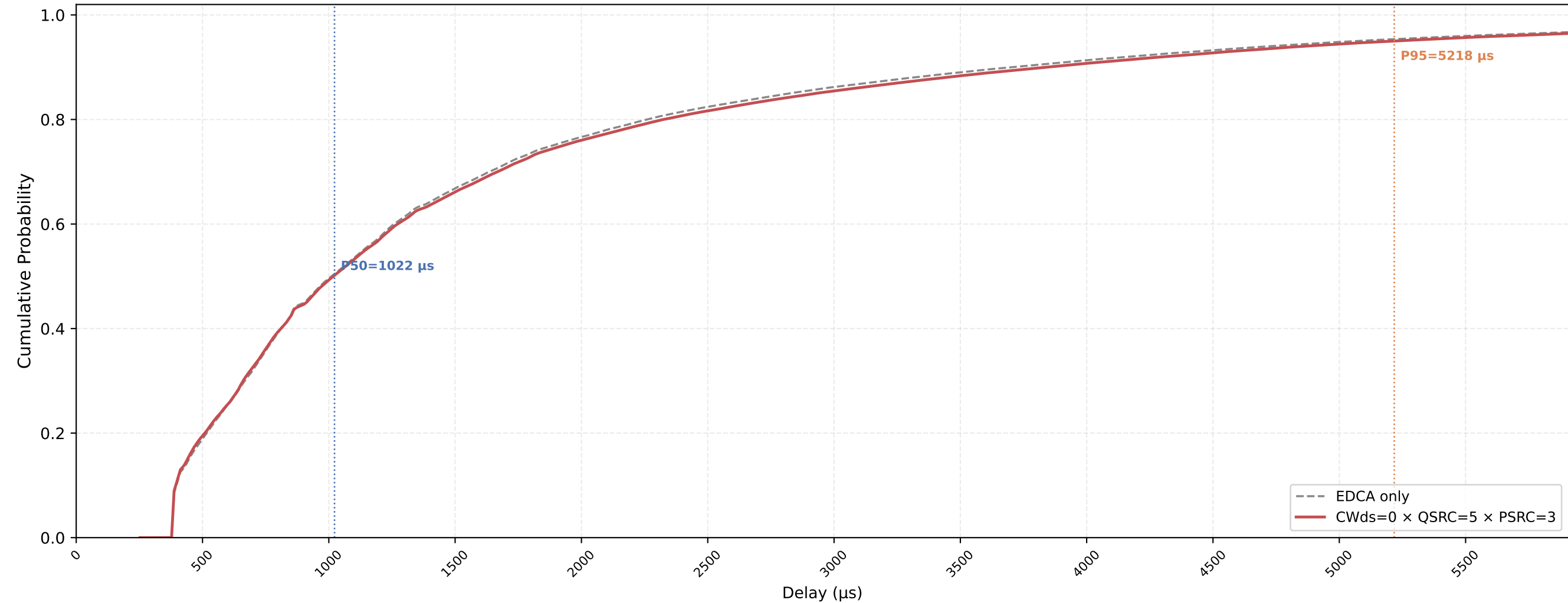
VO (all STAs) Delay CDF — CWds=0 × QSRC=5 × PSRC=3 nSta=30, nPedca=15, 0.5Mbps, avg of 10 runs
