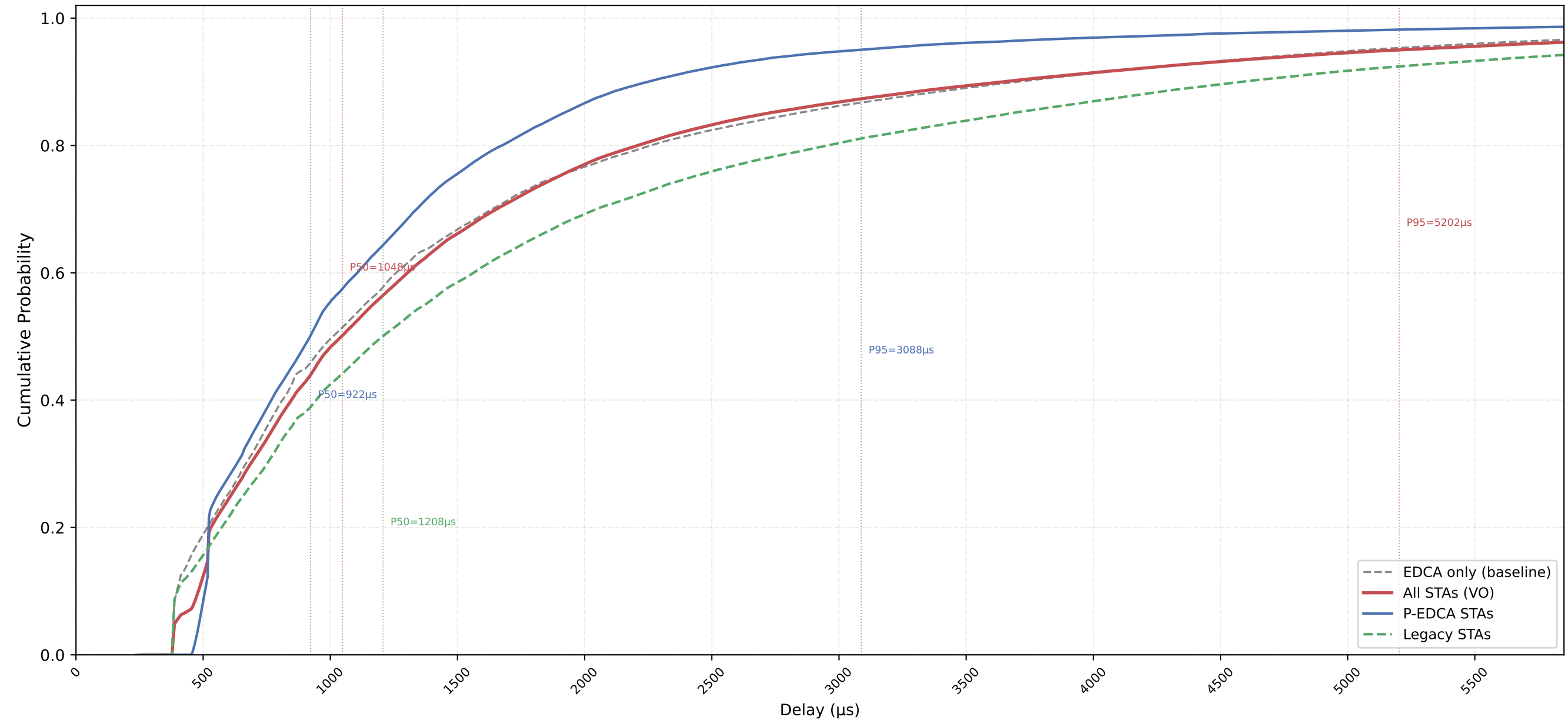
VO Delay CDF — P-EDCA / Legacy / All | CWds=1 × QSRC=0 × PSRC=1 nSta=30, nPedca=15/30, 0.5Mbps, avg of 10 runs
