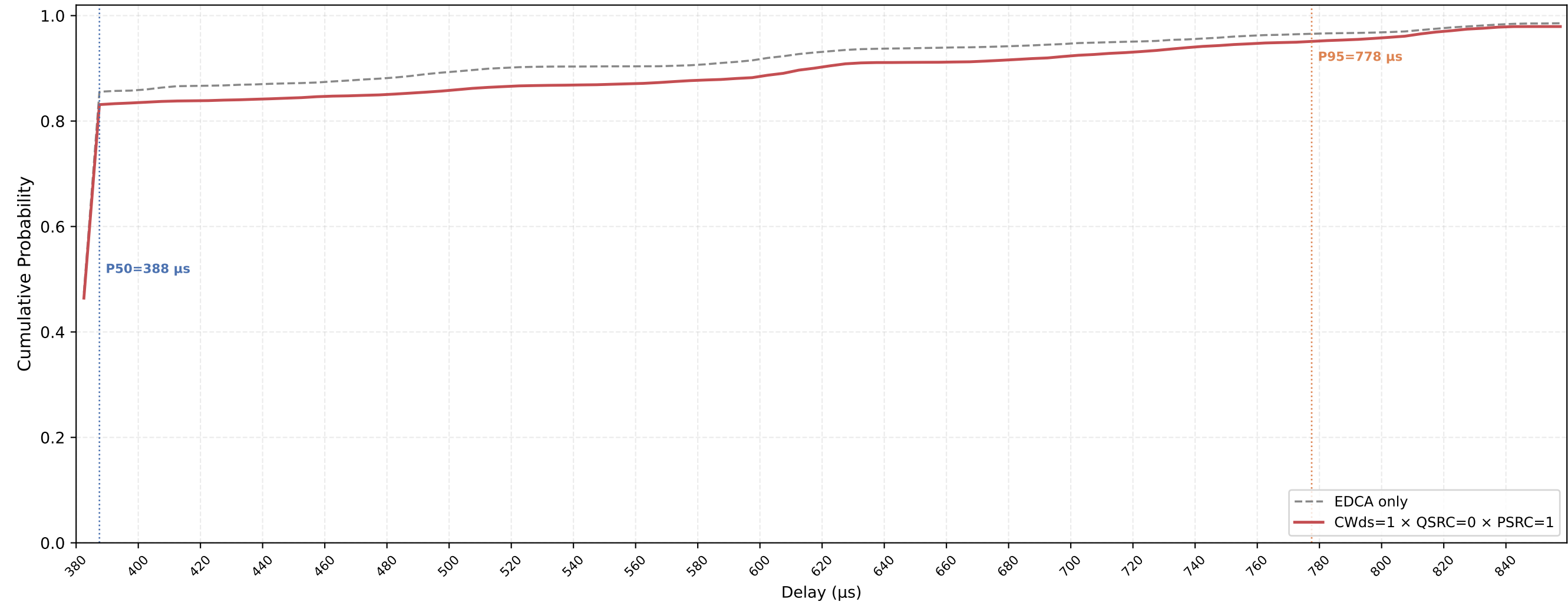
Legacy STA VO Delay CDF — CWds=1 × QSRC=0 × PSRC=1 nSta=30, nPedca=15, 0.1Mbps, avg of 10 runs
