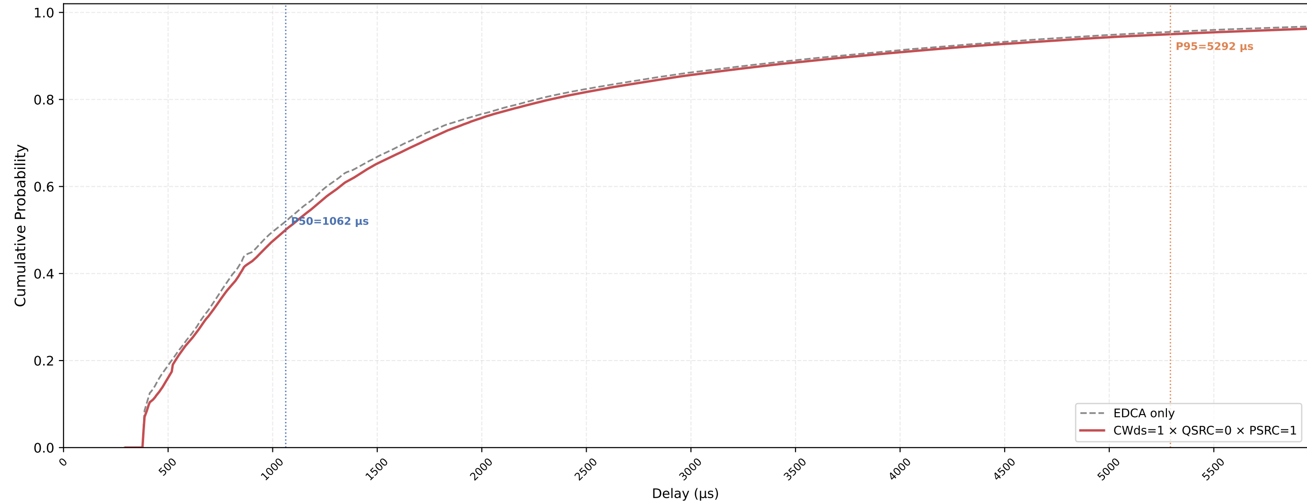
VO (all STAs) Delay CDF — CWds=1 × QSRC=0 × PSRC=1 nSta=30, nPedca=5, 0.5Mbps, avg of 10 runs
