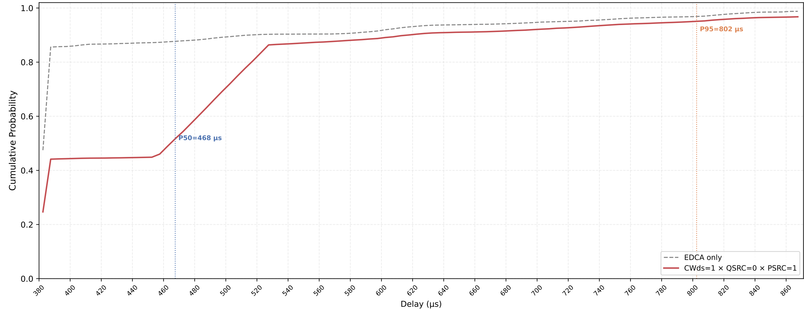
VO (all STAs) Delay CDF — CWds=1 × QSRC=0 × PSRC=1 nSta=30, nPedca=15, 0.1Mbps, avg of 10 runs
