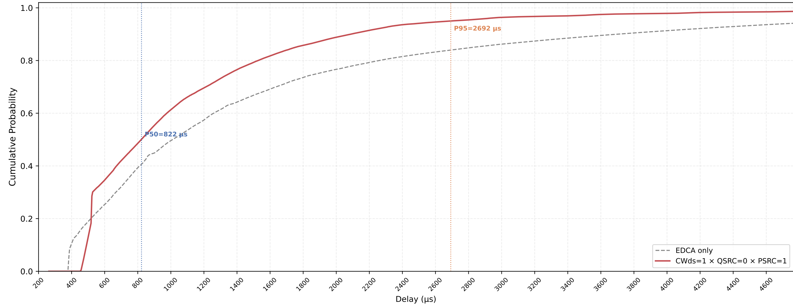
VO (all STAs) Delay CDF — CWds=1 × QSRC=0 × PSRC=1 nSta=30, nPedca=30, 0.5Mbps, avg of 10 runs
