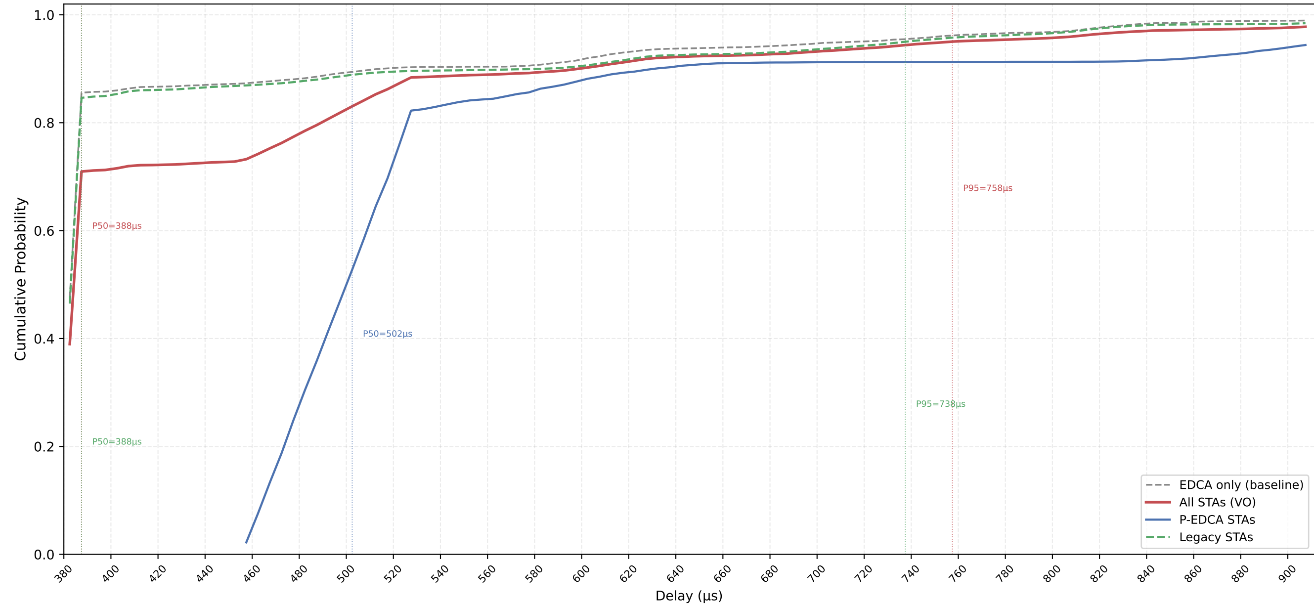
VO Delay CDF — P-EDCA / Legacy / All | CWds=1 × QSRC=0 × PSRC=2 nSta=30, nPedca=5/30, 0.1Mbps, avg of 10 runs
