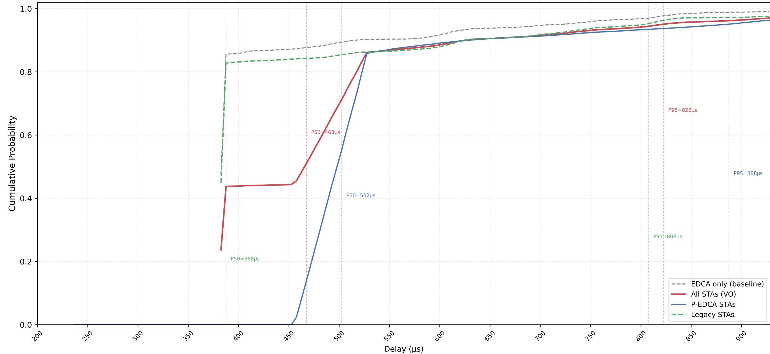
VO Delay CDF — P-EDCA / Legacy / All | CWds=1 × QSRC=0 × PSRC=2 nSta=30, nPedca=15/30, 0.1Mbps, avg of 10 runs
