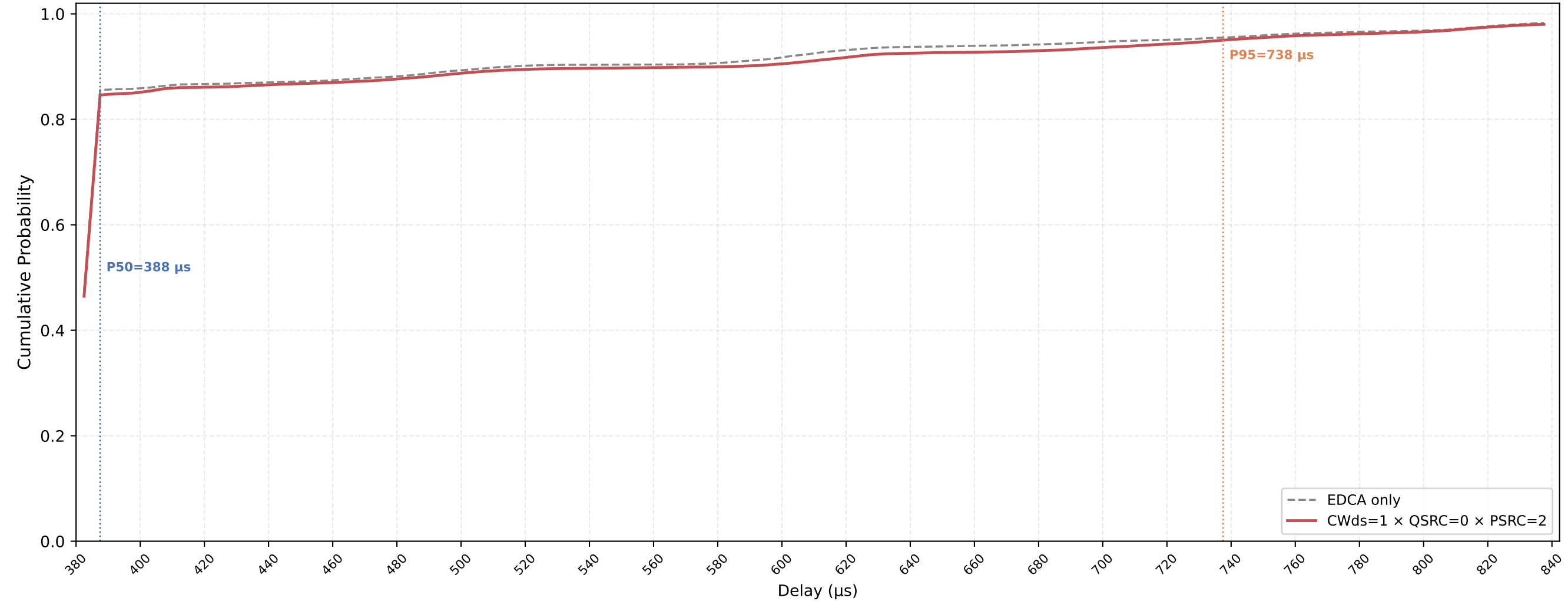
Legacy STA VO Delay CDF — CWds=1 × QSRC=0 × PSRC=2 nSta=30, nPedca=5, 0.1Mbps, avg of 10 runs
