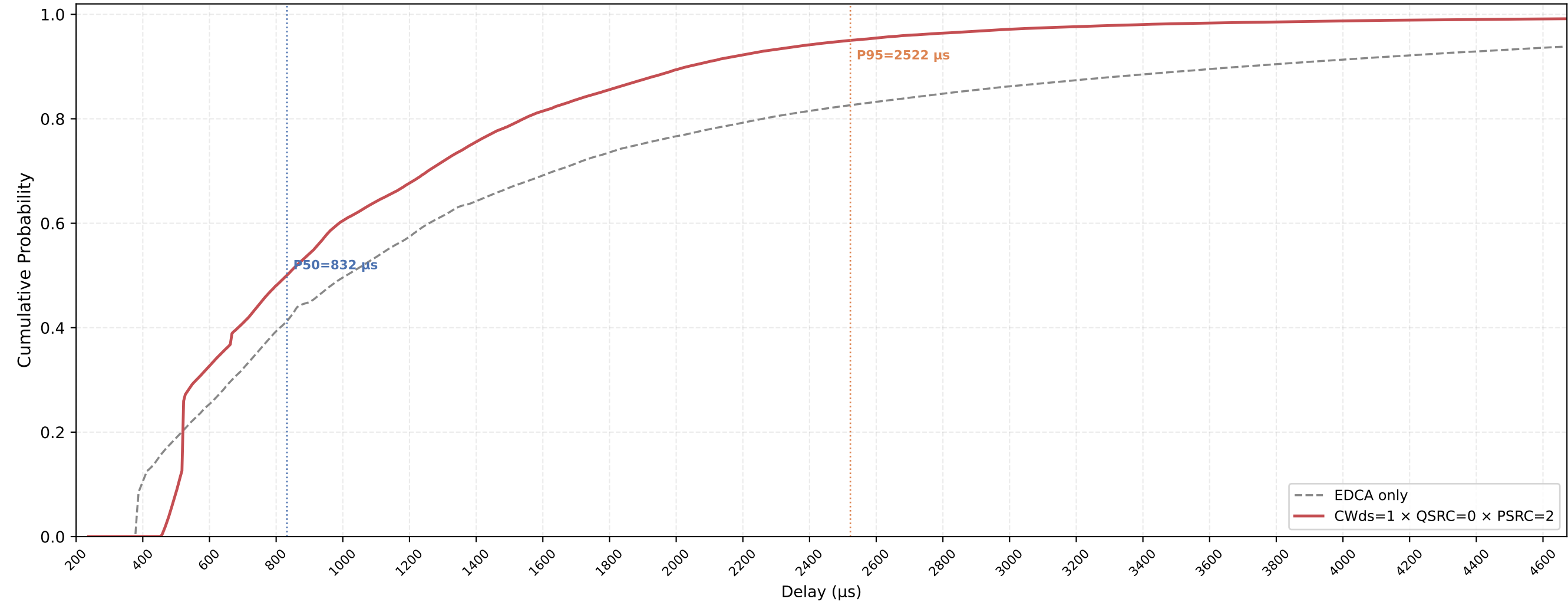
P-EDCA STA VO Delay CDF — CWds=1 × QSRC=0 × PSRC=2 nSta=30, nPedca=15, 0.5Mbps, avg of 10 runs
