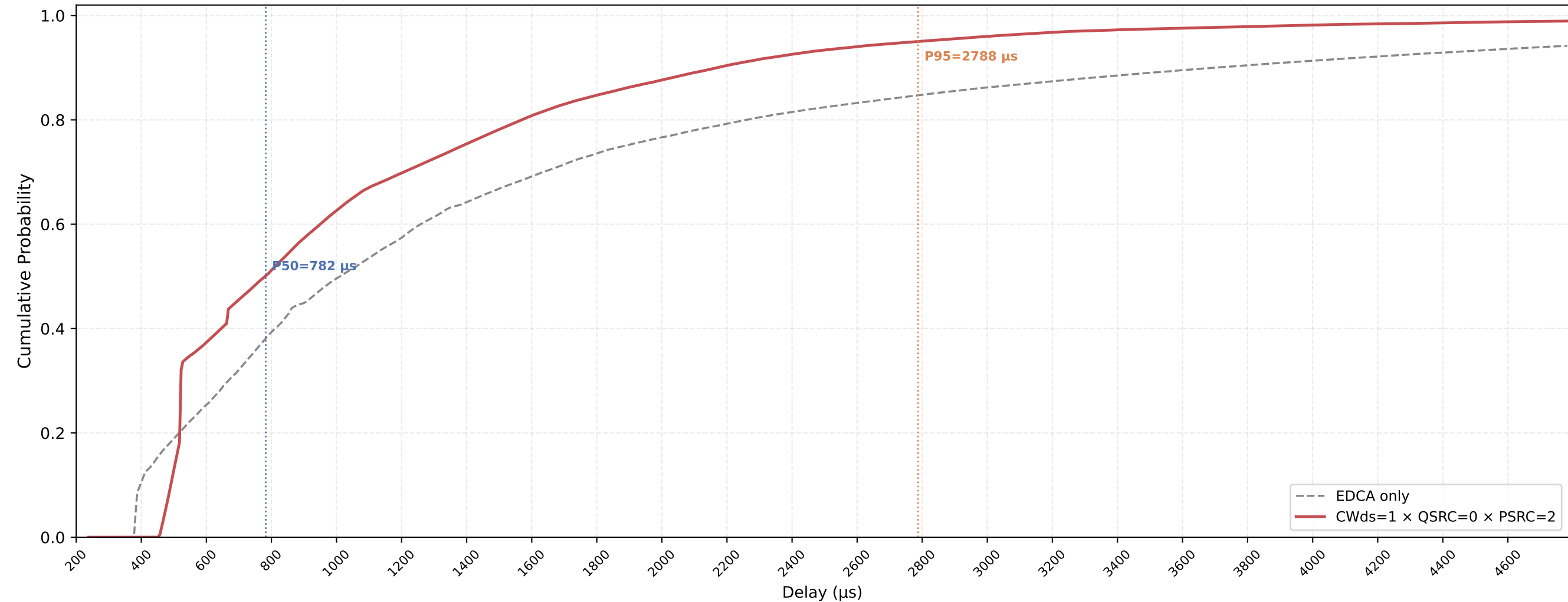
P-EDCA STA VO Delay CDF — CWds=1 × QSRC=0 × PSRC=2 nSta=30, nPedca=30, 0.5Mbps, avg of 10 runs
