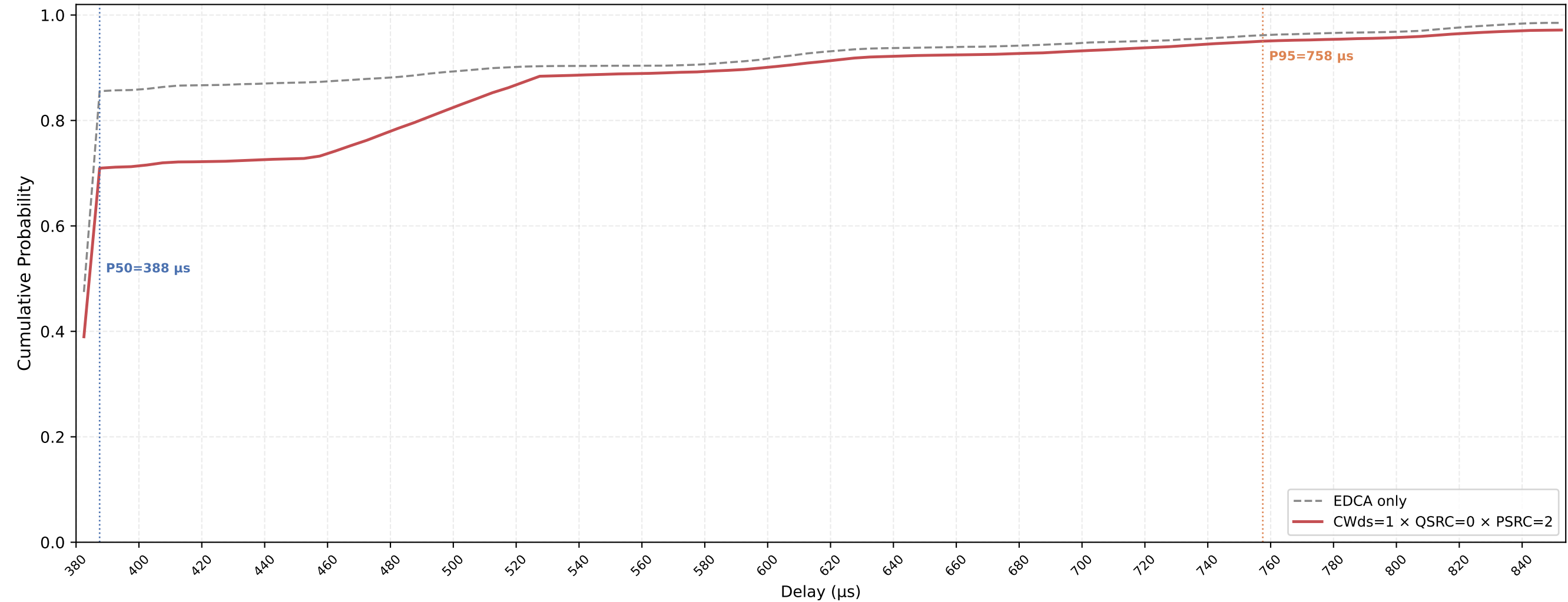
VO (all STAs) Delay CDF — CWds=1 × QSRC=0 × PSRC=2 nSta=30, nPedca=5, 0.1Mbps, avg of 10 runs
