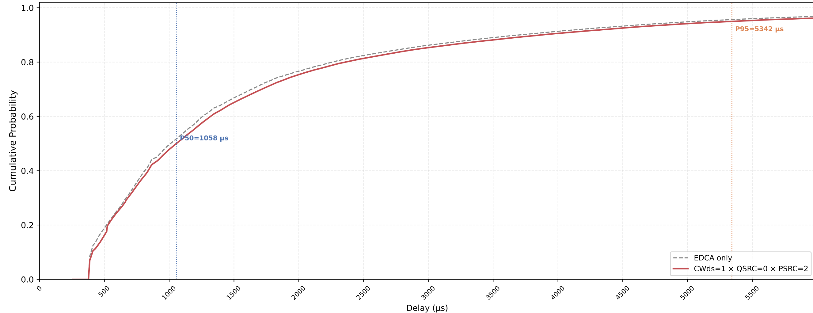
VO (all STAs) Delay CDF — CWds=1 × QSRC=0 × PSRC=2 nSta=30, nPedca=5, 0.5Mbps, avg of 10 runs
