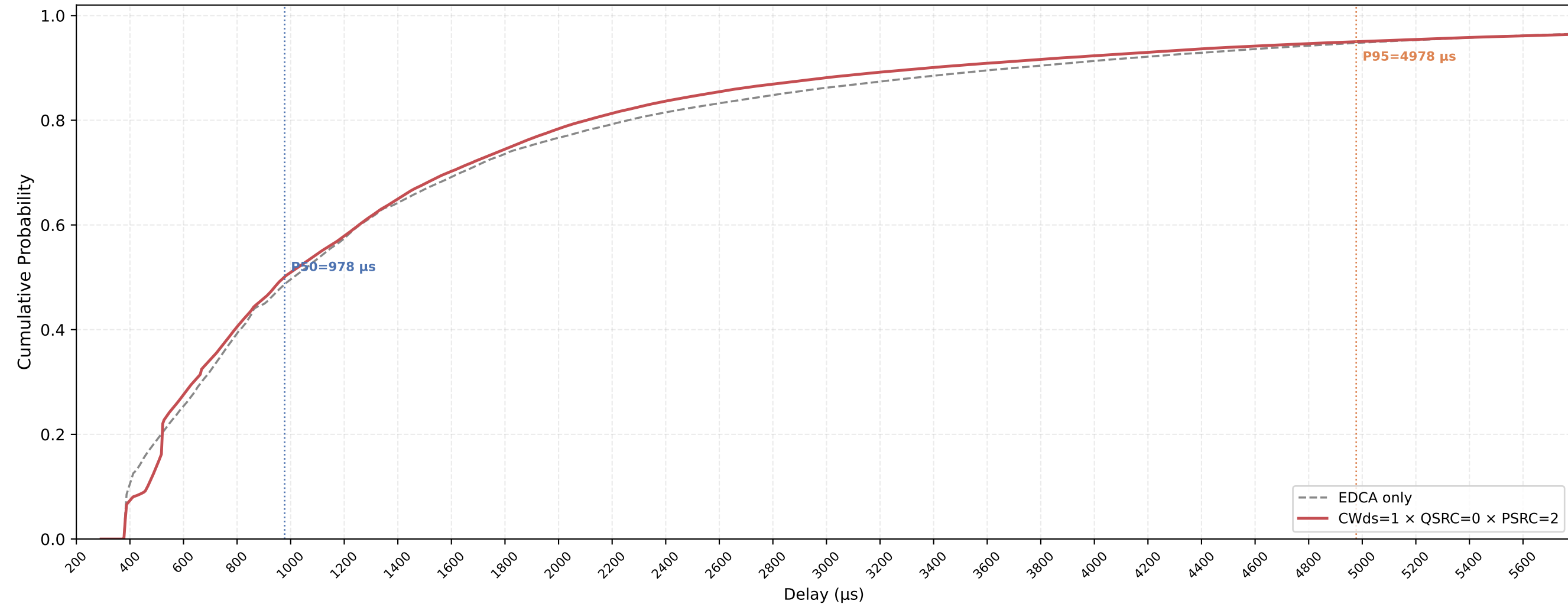
VO (all STAs) Delay CDF — CWds=1 × QSRC=0 × PSRC=2 nSta=30, nPedca=15, 0.5Mbps, avg of 10 runs
