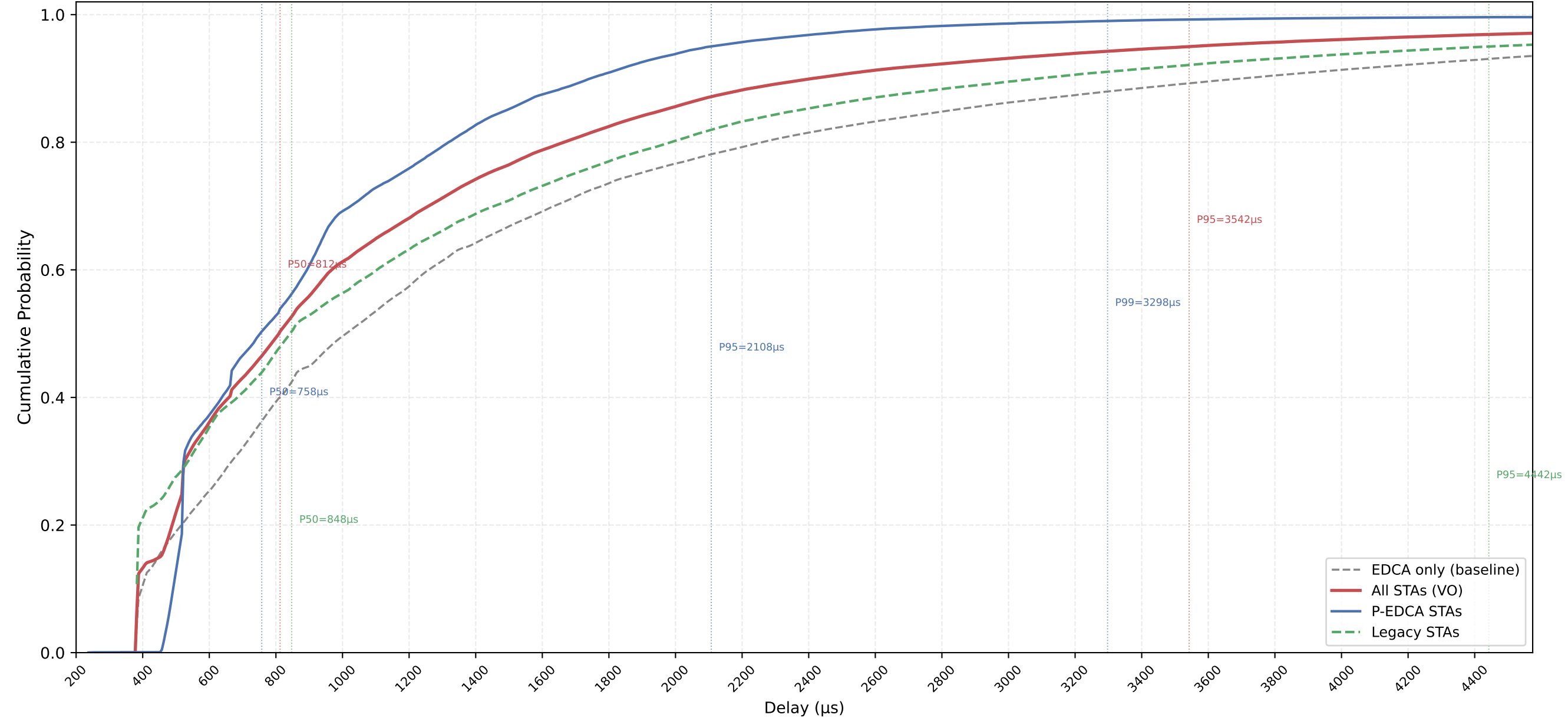
VO Delay CDF — P-EDCA / Legacy / All | CWds=1 × QSRC=0 × PSRC=3 nSta=30, nPedca=15/30, 0.5Mbps, avg of 10 runs
