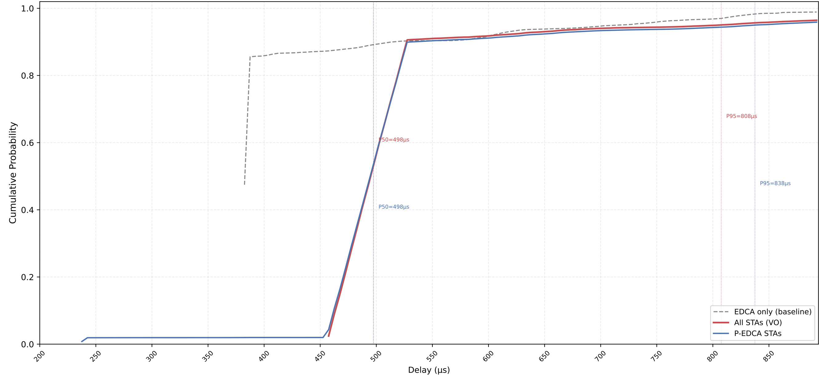
VO Delay CDF — P-EDCA / Legacy / All | CWds=1 × QSRC=0 × PSRC=3 nSta=30, nPedca=30/30, 0.1Mbps, avg of 10 runs
