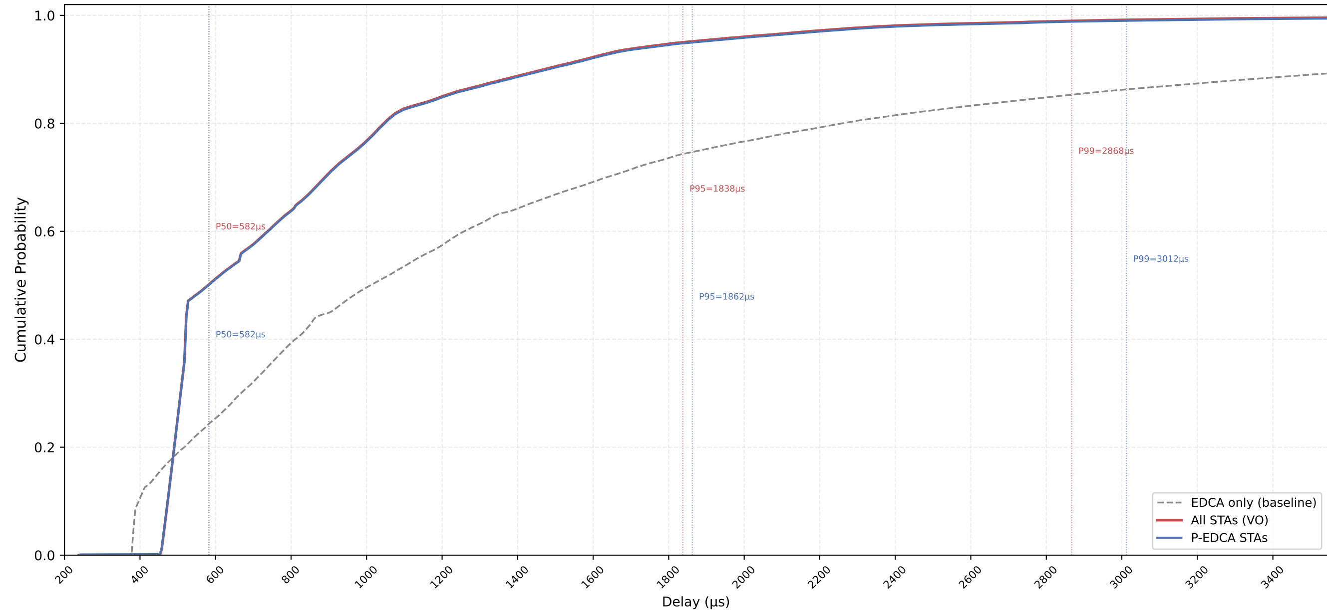
VO Delay CDF — P-EDCA / Legacy / All | CWds=1 × QSRC=0 × PSRC=3 nSta=30, nPedca=30/30, 0.5Mbps, avg of 10 runs
