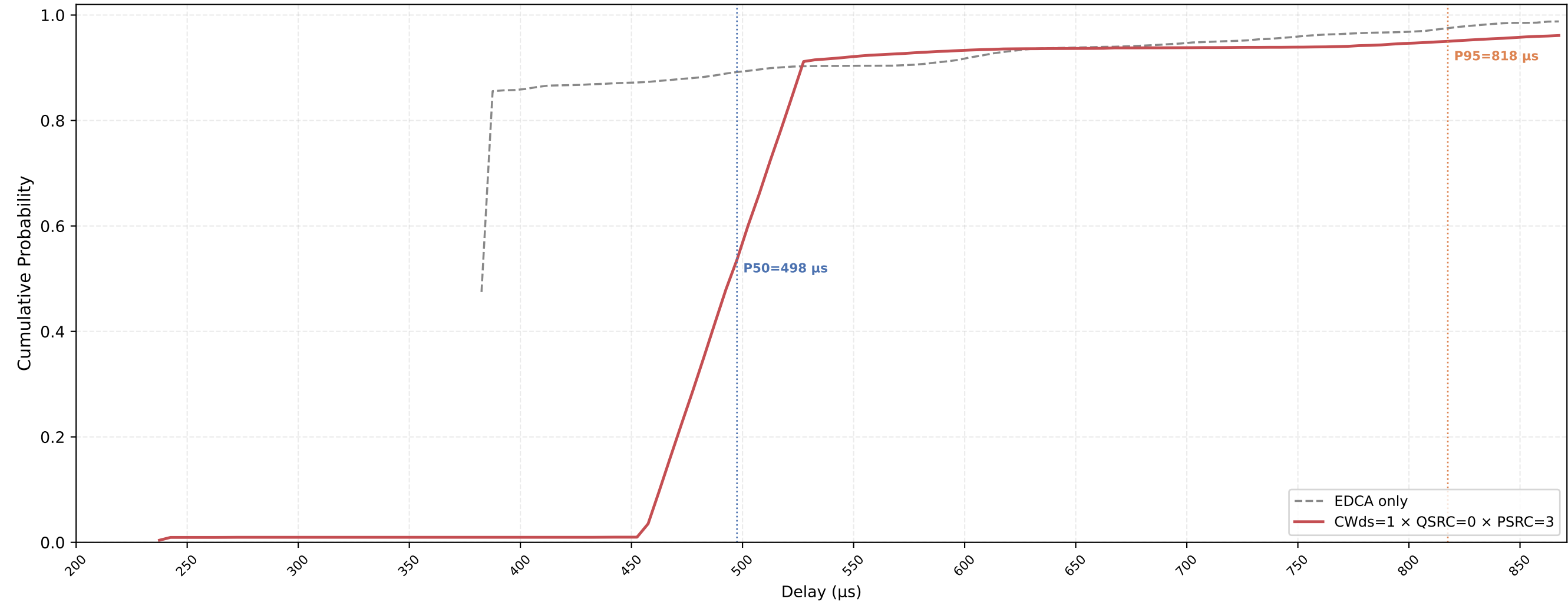
P-EDCA STA VO Delay CDF — CWds=1 × QSRC=0 × PSRC=3 nSta=30, nPedca=15, 0.1Mbps, avg of 10 runs
