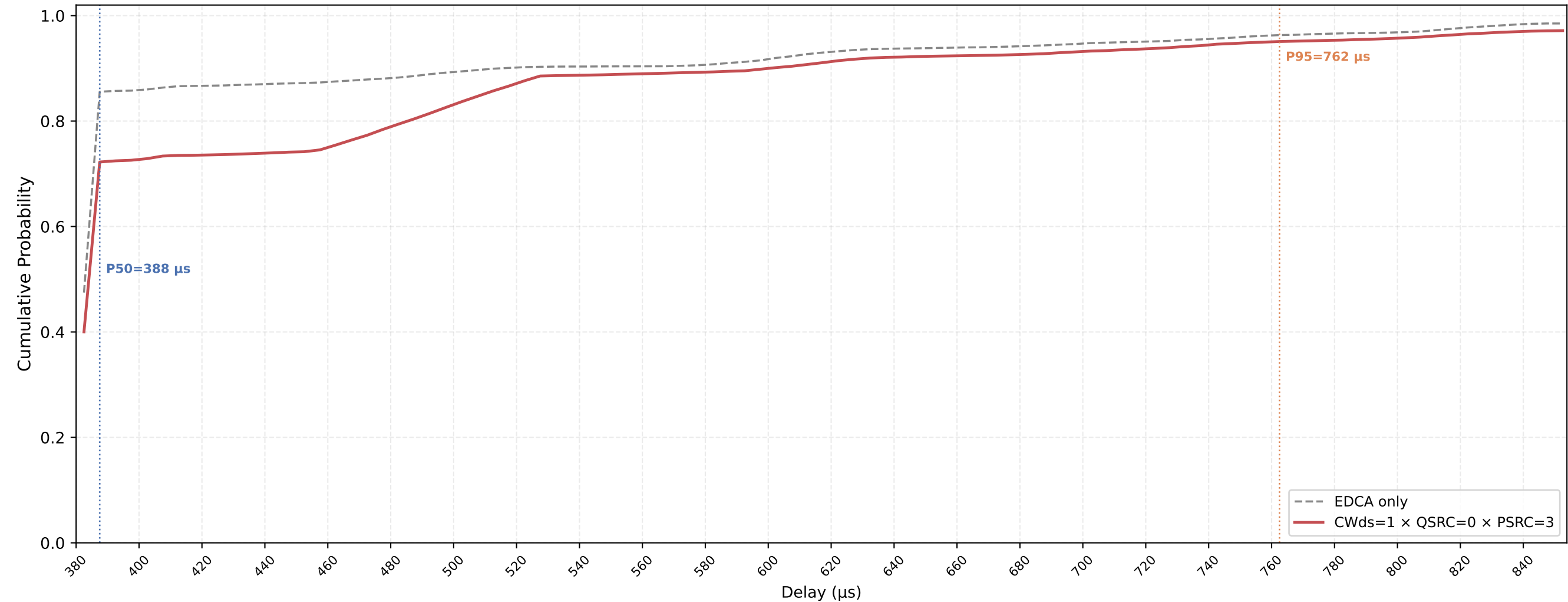
VO (all STAs) Delay CDF — CWds=1 × QSRC=0 × PSRC=3 nSta=30, nPedca=5, 0.1Mbps, avg of 10 runs
