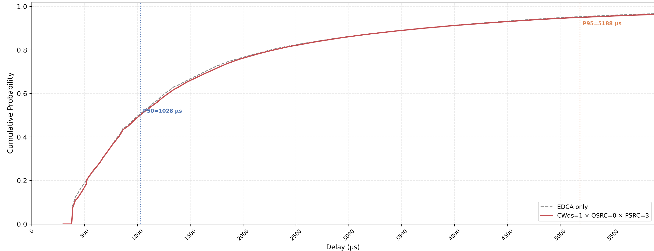
VO (all STAs) Delay CDF — CWds=1 × QSRC=0 × PSRC=3 nSta=30, nPedca=5, 0.5Mbps, avg of 10 runs
