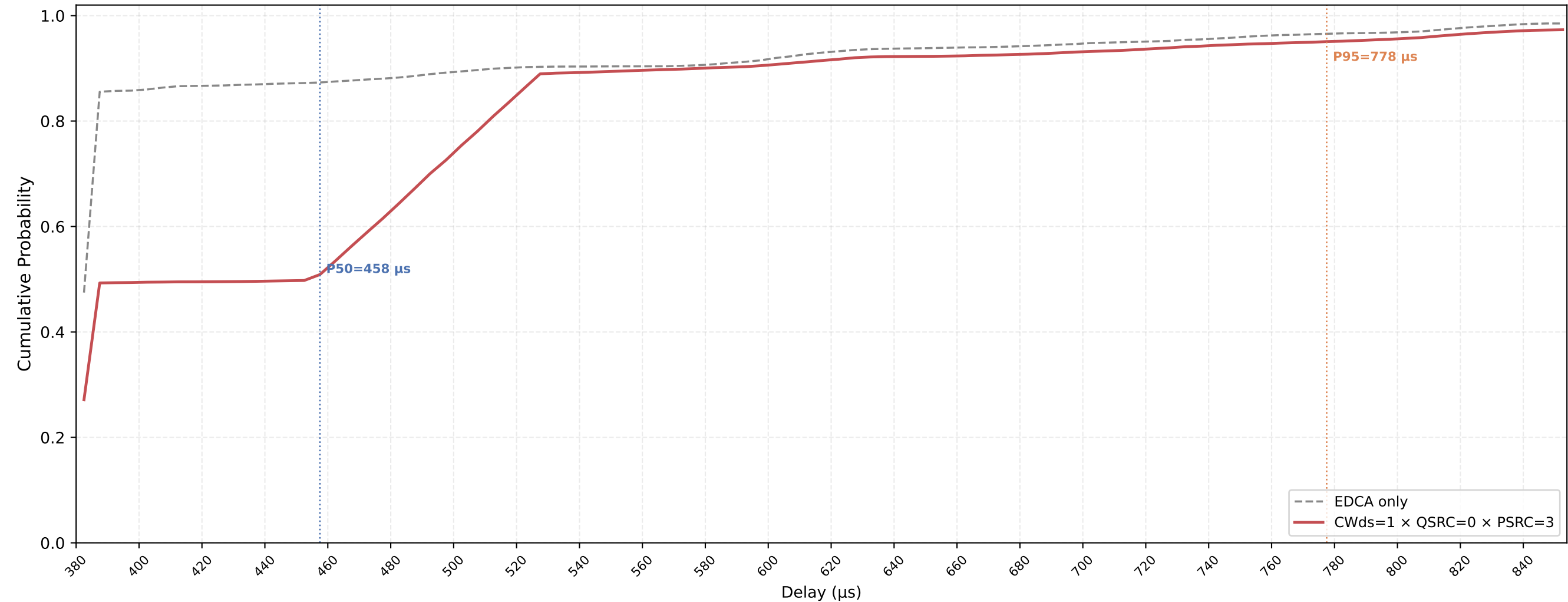
VO (all STAs) Delay CDF — CWds=1 × QSRC=0 × PSRC=3 nSta=30, nPedca=15, 0.1Mbps, avg of 10 runs
