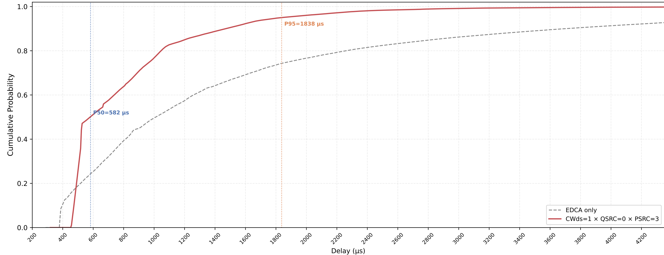
VO (all STAs) Delay CDF — CWds=1 × QSRC=0 × PSRC=3 nSta=30, nPedca=30, 0.5Mbps, avg of 10 runs
