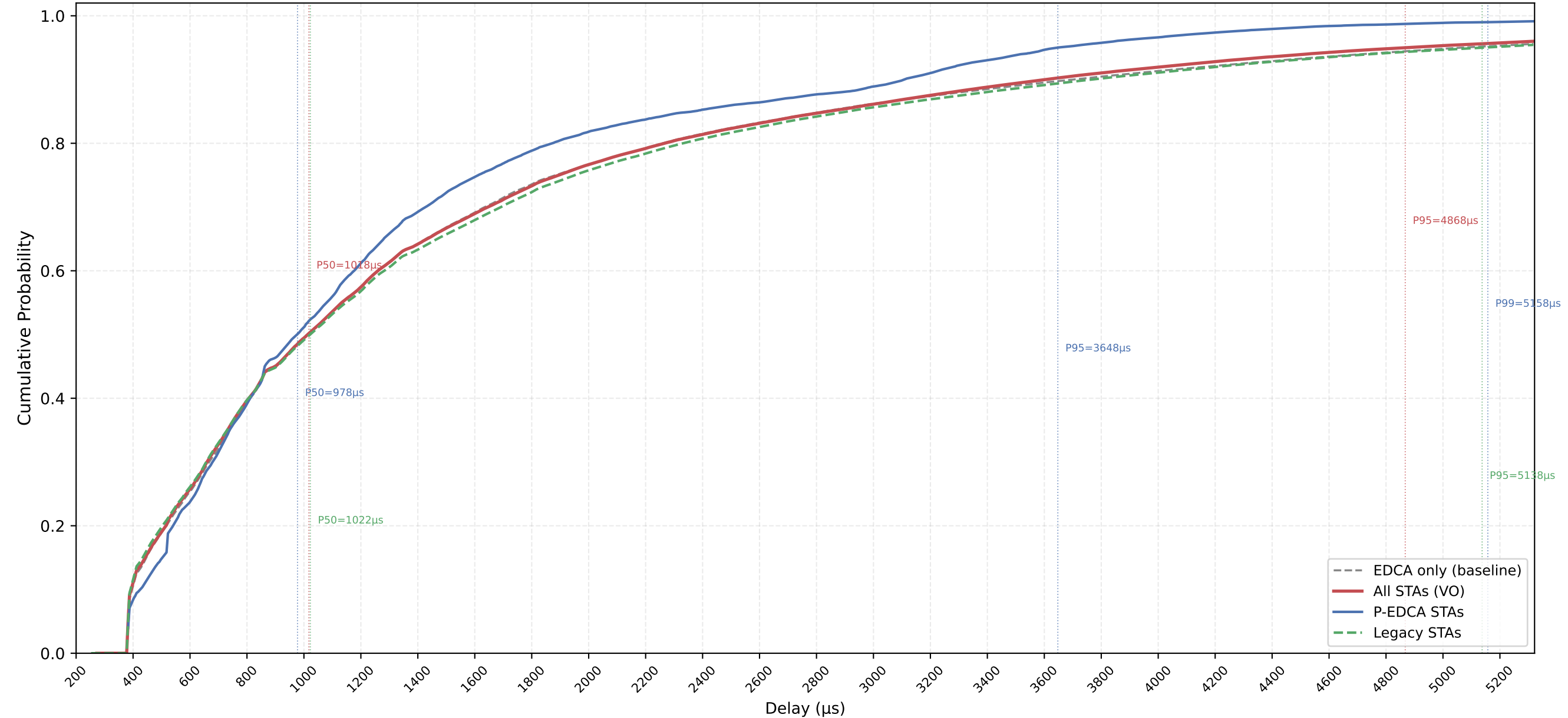
VO Delay CDF — P-EDCA / Legacy / All | CWds=1 × QSRC=1 × PSRC=1 nSta=30, nPedca=5/30, 0.5Mbps, avg of 10 runs
