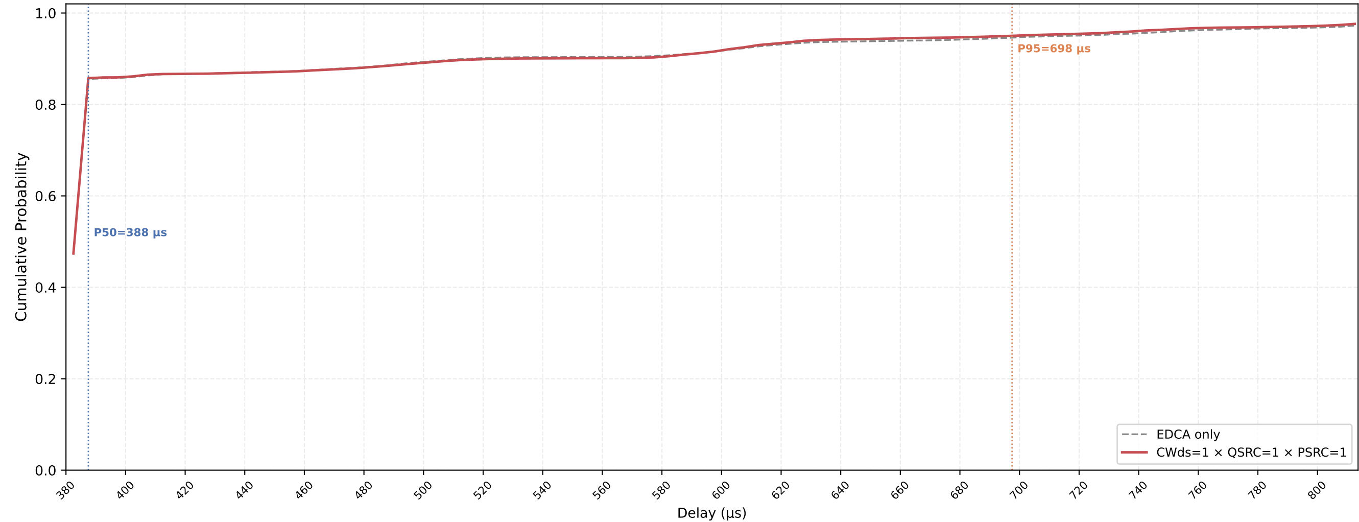
Legacy STA VO Delay CDF — CWds=1 × QSRC=1 × PSRC=1 nSta=30, nPedca=5, 0.1Mbps, avg of 10 runs
