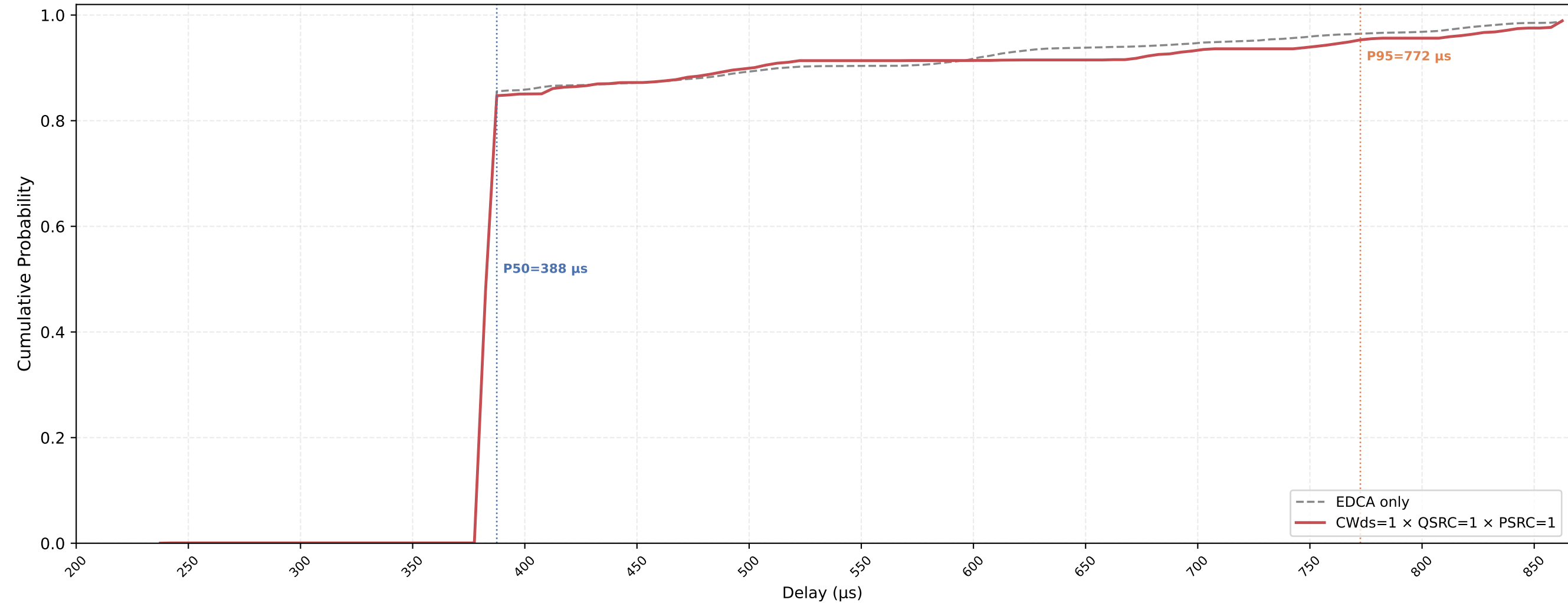
P-EDCA STA VO Delay CDF — CWds=1 × QSRC=1 × PSRC=1 nSta=30, nPedca=5, 0.1Mbps, avg of 10 runs
