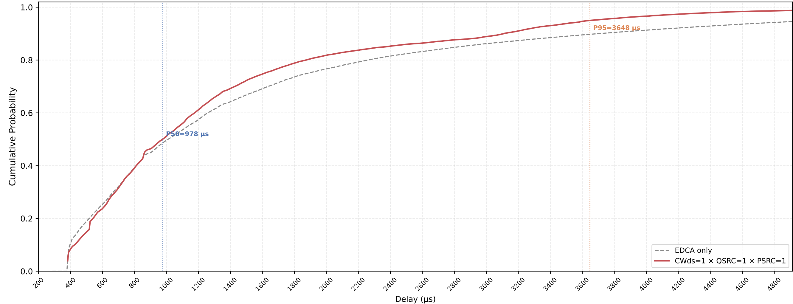
P-EDCA STA VO Delay CDF — CWds=1 × QSRC=1 × PSRC=1 nSta=30, nPedca=5, 0.5Mbps, avg of 10 runs
