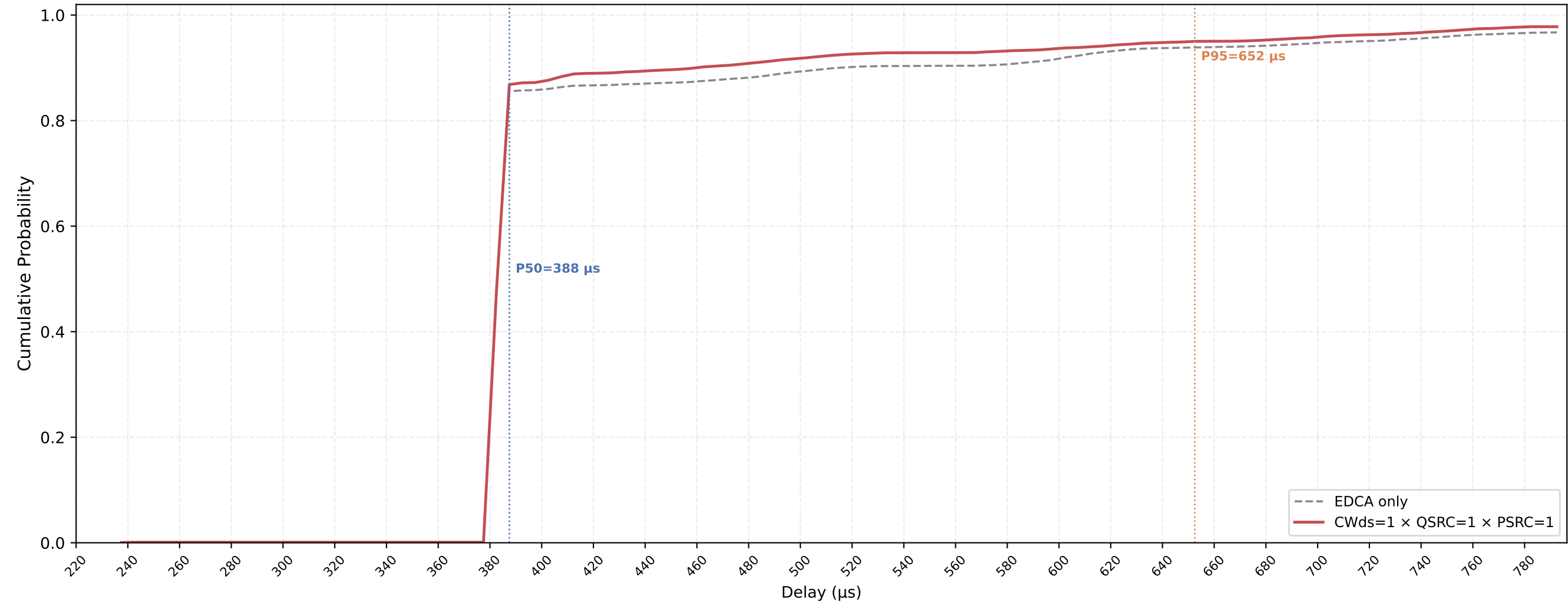
P-EDCA STA VO Delay CDF — CWds=1 × QSRC=1 × PSRC=1 nSta=30, nPedca=15, 0.1Mbps, avg of 10 runs
