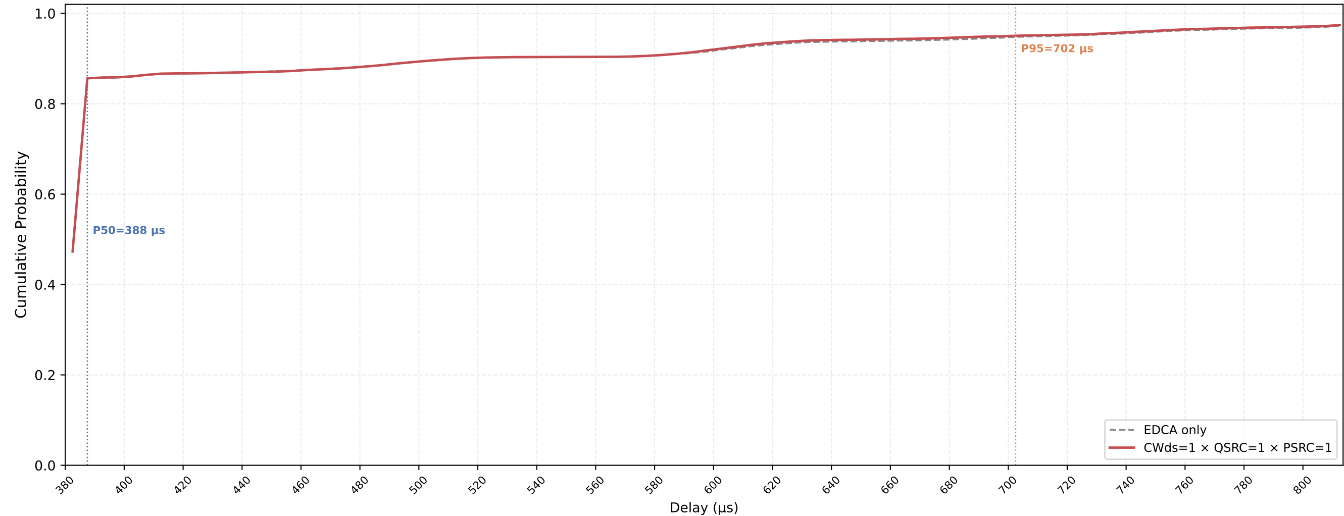
VO (all STAs) Delay CDF — CWds=1 × QSRC=1 × PSRC=1 nSta=30, nPedca=15, 0.1Mbps, avg of 10 runs
