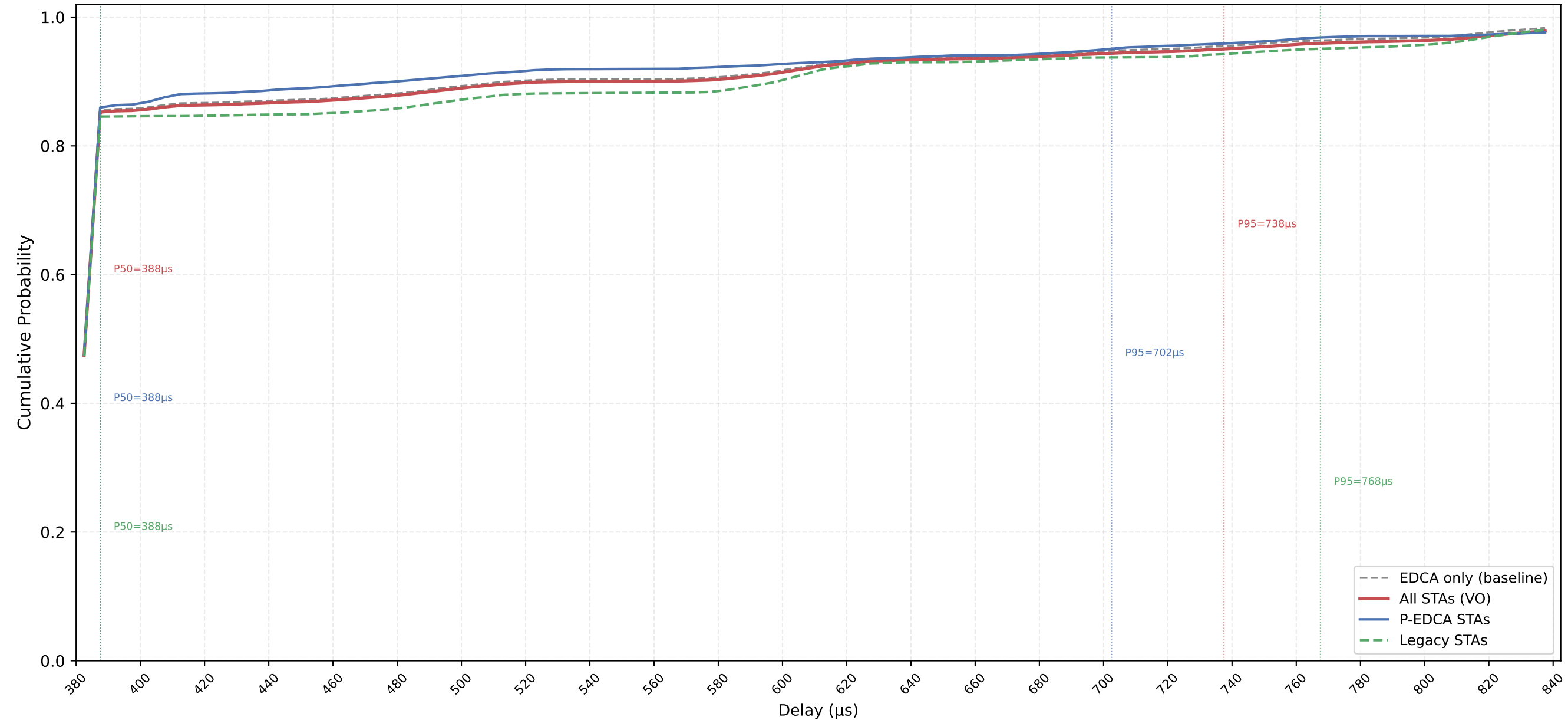
VO Delay CDF — P-EDCA / Legacy / All | CWds=1 × QSRC=1 × PSRC=2 nSta=30, nPedca=15/30, 0.1Mbps, avg of 10 runs
