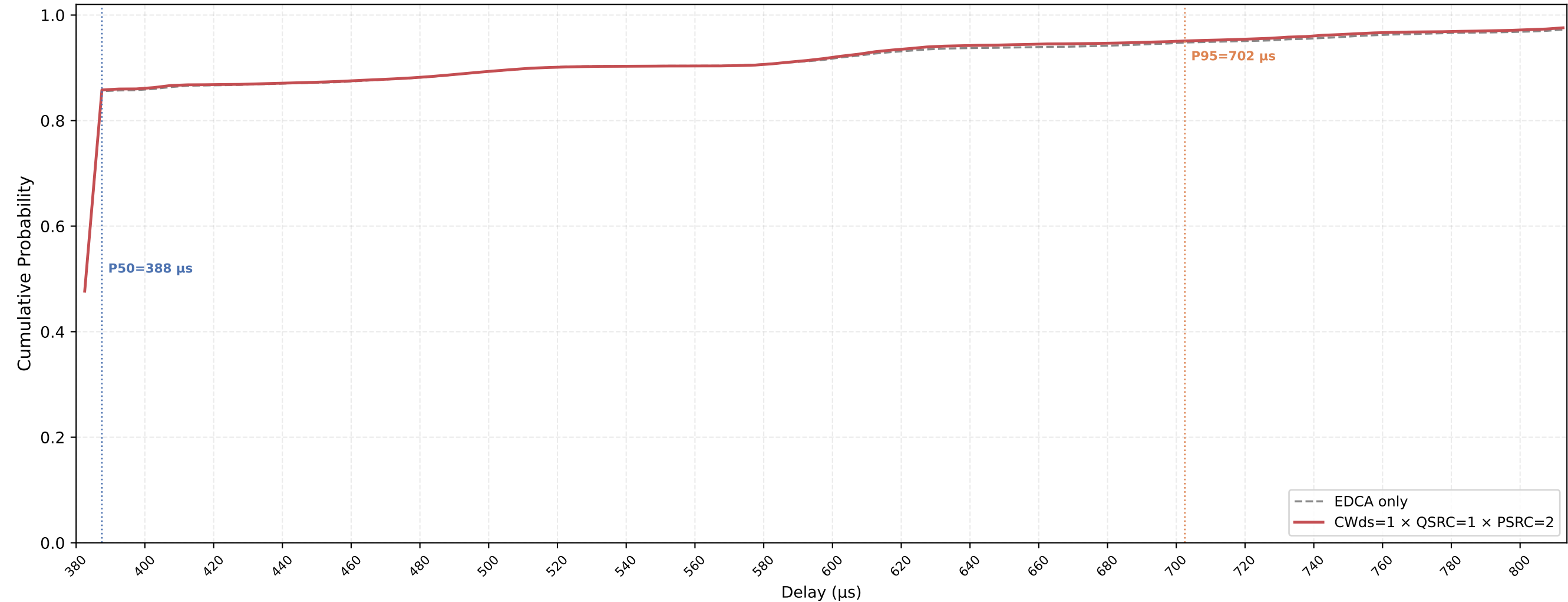
Legacy STA VO Delay CDF — CWds=1 × QSRC=1 × PSRC=2 nSta=30, nPedca=5, 0.1Mbps, avg of 10 runs
