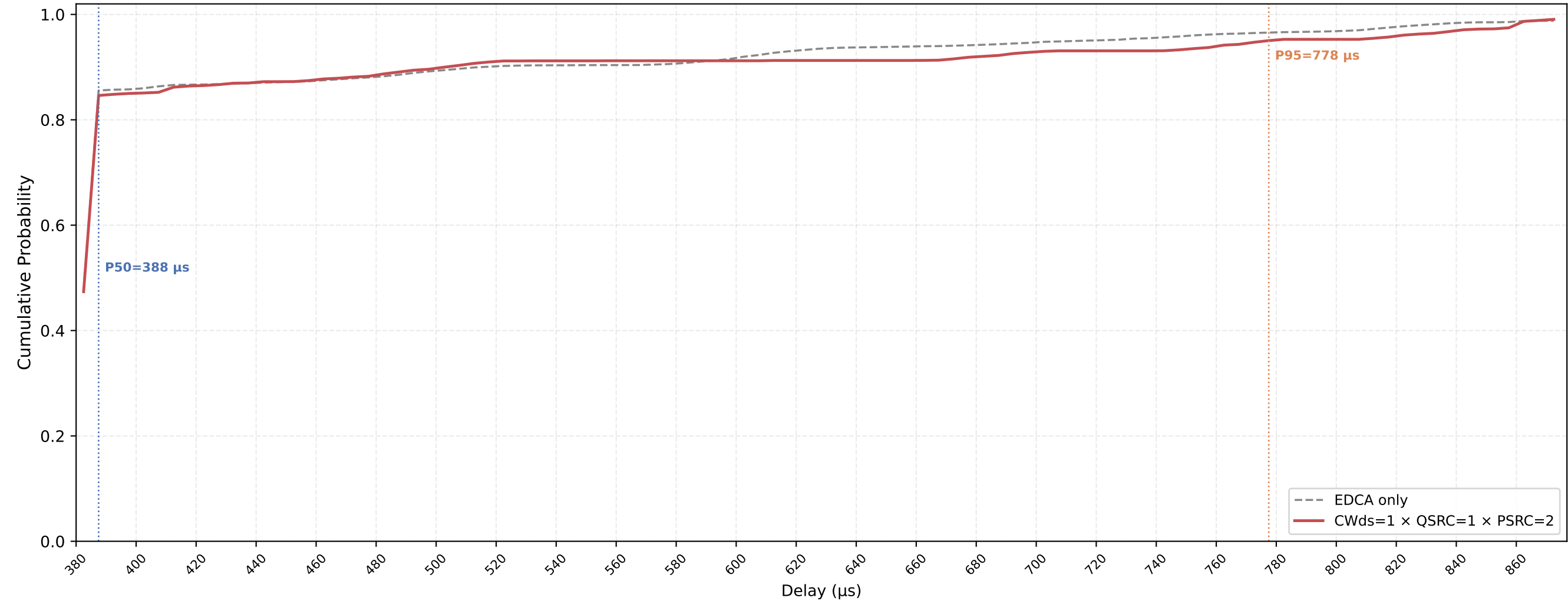
P-EDCA STA VO Delay CDF — CWds=1 × QSRC=1 × PSRC=2 nSta=30, nPedca=5, 0.1Mbps, avg of 10 runs
