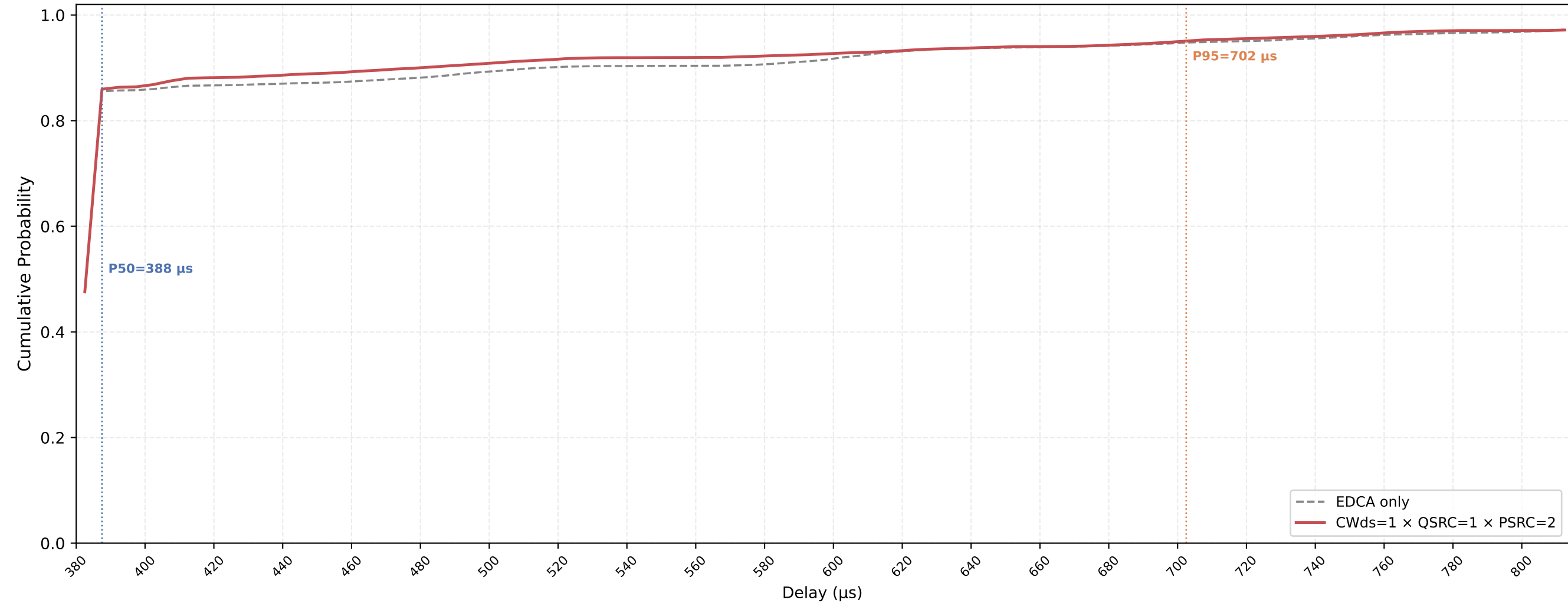
P-EDCA STA VO Delay CDF — CWds=1 × QSRC=1 × PSRC=2 nSta=30, nPedca=15, 0.1Mbps, avg of 10 runs
